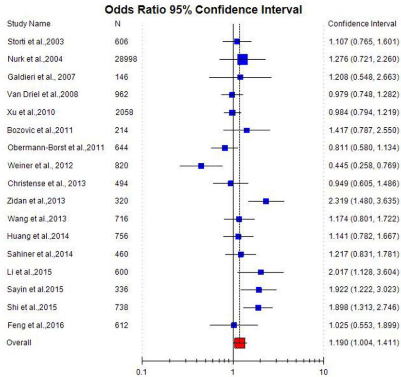
Figure 1: Forest plots (random effect) of allele contrast model (C versus A) showed significant association between maternal MTHFR A1298C polymorphism and CHD risk.
