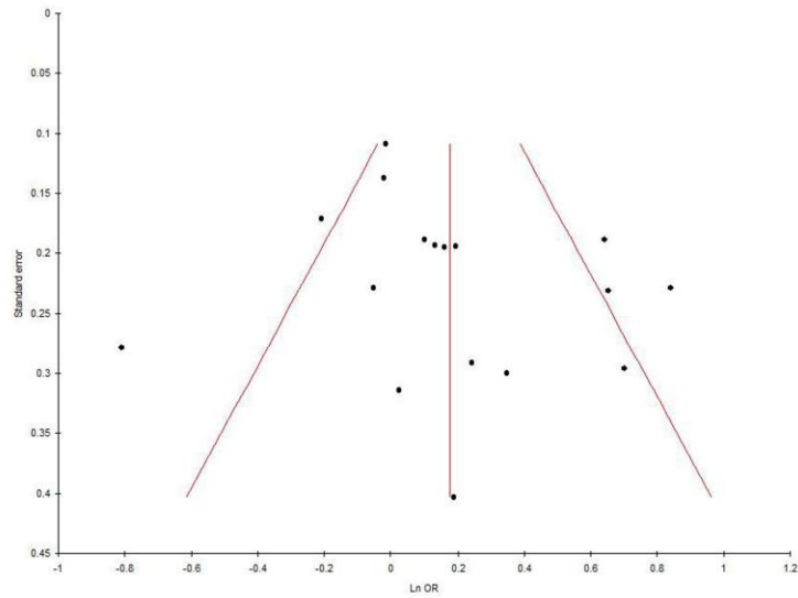
Figure 6. Funnel plots of standard error by OR of MTHFR A1298C allele contrast
