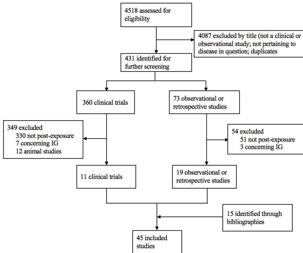
Figure 1: Study selection
