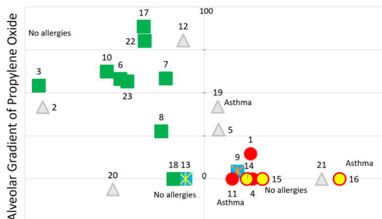
Figure 2 Scatter plot showing a composite score derived from five VOCs, reflecting the progression of inflammatory response, plotted against the alveolar gradient of Propylene Oxide
