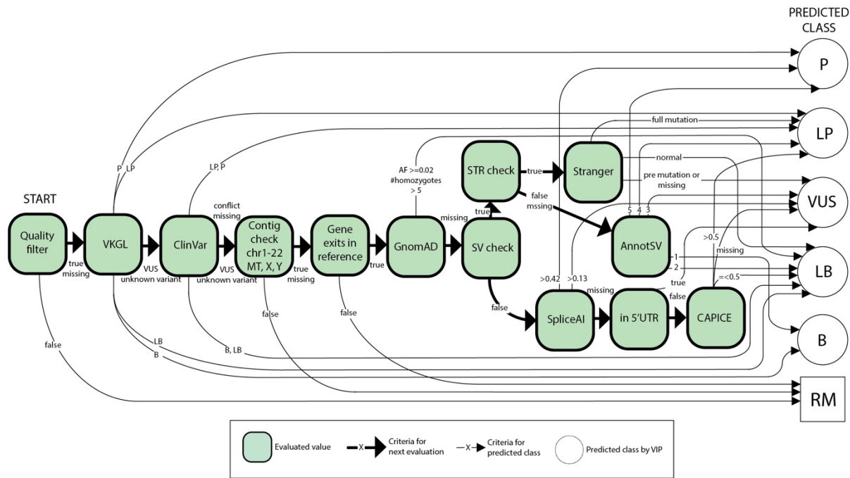
Figure 2 Default decision tree . The figure shows a schematic version of the default decision tree. The green blocks and bold arrows represent the general sequence of filtering steps and the values that are evaluated for each variant (see legend). Each value is calculated in the annotation module (supplementary table 1). Small arrows represent the decisions for the consequence classifications by VIP. VIP classifies the different consequences as B, LB, VUS, LP or P. After a variant is classified by VIP, it exits the filter tree. Variants with incorrect contigs or genes and low quality are removed (RM). Using the JSON format, each component in the decision tree can be customized to fit the workflow of the user.
