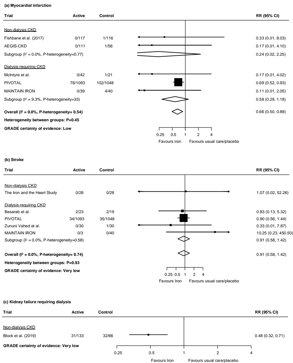
Figure 3. Effects of iron therapies vs. usual care or placebo on (A) myocardial infarction, (B) stroke and (C) kidney failure in people with CKD.
