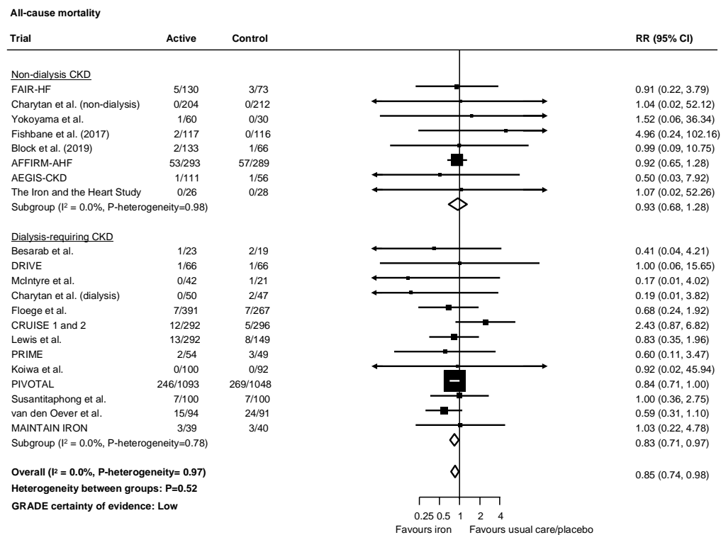
Figure 4. Effect of iron therapies vs. usual care or placebo on all-cause mortality in people with CKD.
