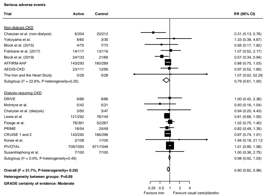
Figure 5. Effect of iron therapies vs. usual care or placebo on serious adverse events in people with CKD.
