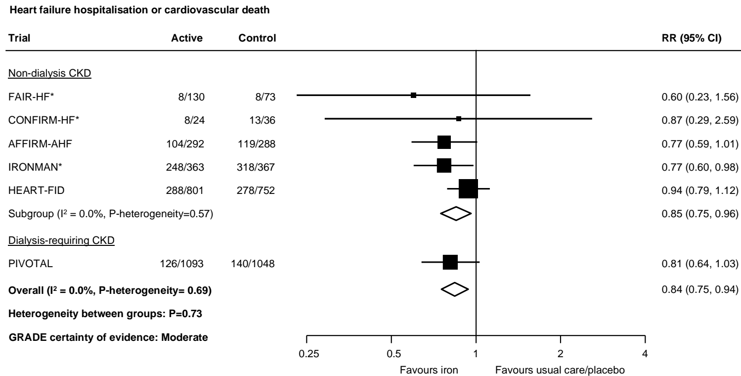
Figure 1. Effect of iron therapies vs. usual care or placebo on hospitalisation for heart failure or cardiovascular death in people with CKD.
