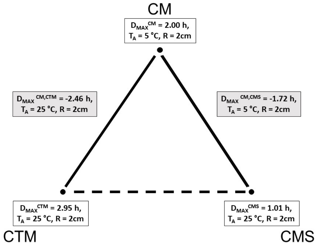
Fig. 10: Maximum TDE deviation in D_{MAX} in CTM, CMS and CM model
