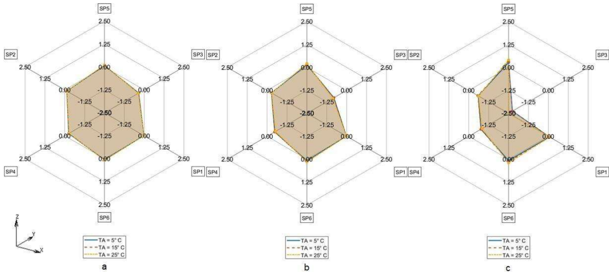
Fig. 9: Difference in TDE deviation in D_{MAX} between CM vs CTM for T_A = 5^\circ\text{C} (Solid line), T_A = 15^\circ\text{C} (Dashed line), T_A = 25^\circ\text{C} (Dash-dotted line) a. R = 0.5\text{ cm} , b. R = 1\text{ cm} , c. R = 2\text{ cm}
