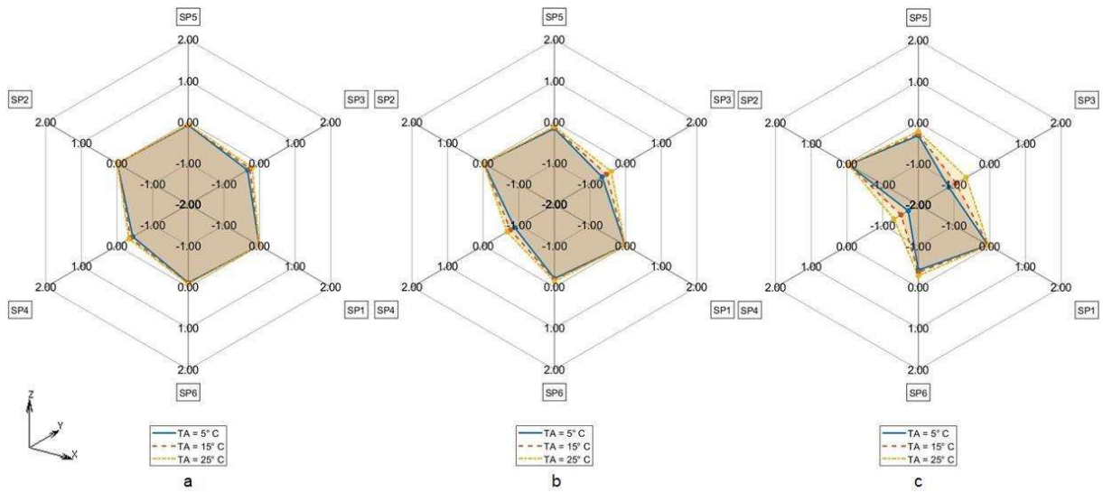
Fig. 8: Difference in TDE deviation in D_{MAX} between CM vs CMS model for T_A = 5^\circ C (Solid line), T_A = 15^\circ C (Dashed line), T_A = 25^\circ C (Dash-dotted line) for a. R = 0.5 cm, b. R = 1 cm, c. R = 2 cm
