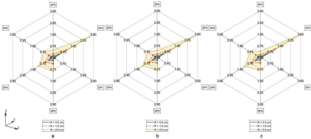
Fig. 5: TDE deviation in D_{MAX} for CTM for R = 0.5 cm (Solid line), R = 1.0 cm (Dashed line), R = 2 cm (Dash-dotted line) a. T_A = 5^\circ C, b. T_A = 15^\circ C, c. T_A = 25^\circ C
