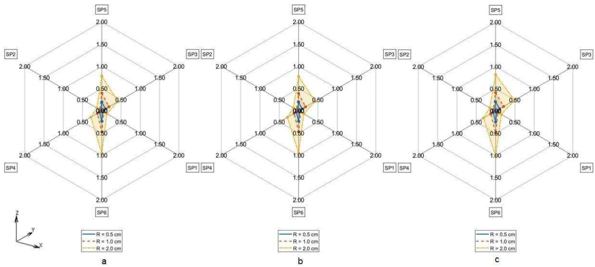
Fig. 7: TDE deviation in D_{MAX} for CM for R = 0.5 cm (Solid line), R = 1.0 cm (Dashed line), R = 2 cm (Dash-dotted line) a. T_A = 5^\circ C, b. T_A = 15^\circ C, c. T_A = 25^\circ C
