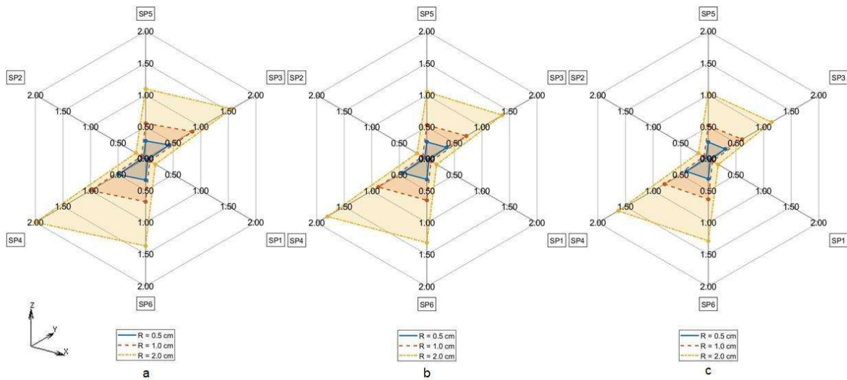
Fig. 6: TDE deviation in D_{MAX} for CMS for R = 0.5 cm (Solid line), R = 1.0 cm (Dashed line), R = 2 cm (Dash-dotted line) a. T_A = 5^\circ C, b. T_A = 15^\circ C, c. T_A = 25^\circ C
