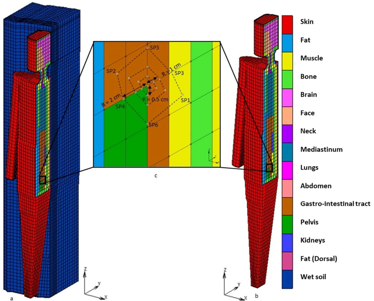
Fig. 2 a: Coarse model lying on a support structure (CMS), Fig. 2 b: Coarse model without support structure (CM), Fig. 2 c: Detailed view of measurement points C, SP 1 ,...,SP 6 along different radii R = 0.5 cm, 1 cm, 2 cm. For the octahedra see Fig.4. Only the contour lines of the octahedra are shown for clarity.
