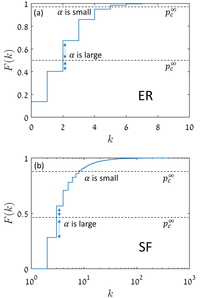
FIG. S2. Examples of F(k) . The decay rate \alpha determines the regimes of power law or exponential convergence of p_c(n \rightarrow \infty) . \alpha depends on the minimal ratio between p_c^{\infty} and F(k) . Hence \alpha is influenced by the density of F(k) in the neighborhood of p_c^{\infty} . Here we show the patterns of F(k) for ER network with N = 10^4 and k = 2 (a), and for SF network with N = 10^4 and \gamma = 2.5 (b). One can see that for larger p_c^{\infty} , F(k) is much more dense for SF network, which makes \alpha become small and extend the power-law regime.
