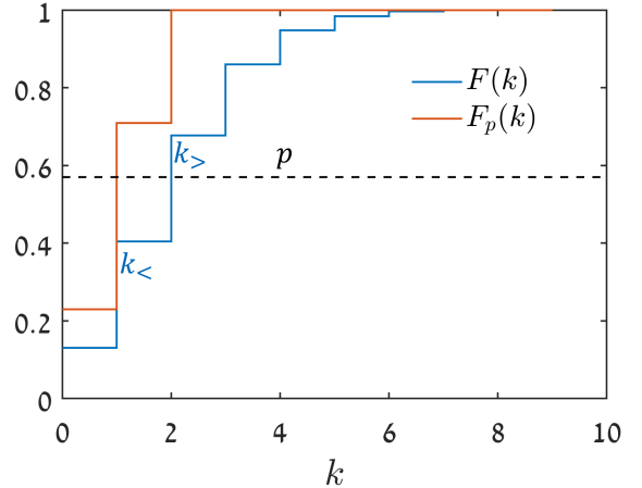
FIG. S1. Illustration of theory for F_p(k) for large n . For small k , F(k) < p , F_p(k) \rightarrow F(k)/p , and for large k , F(k) > p , F_p(k) \rightarrow 1 . The dashed horizontal line is at the value of p . k_< and k_> are the consecutive degrees for which F(k_<) < p < F(k_>) respectively. For determining the decay rate \alpha in Eq. (S17), one should take p = p_c , and find the minimum of |\log(F(k)/p_c^\infty)| among all k , which is in fact among k_< and k_> .
