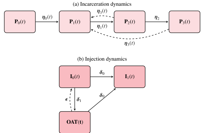
Figure S1.2: (a) People who initiate injection have never been incarcerated ( P_0(t) ) and can be incarcerated at a time-dependent rate \eta_0(t) . They are then released back to the community at a time-dependent rate \eta_1(t) and are considered recently released for 6 months ( P_2(t) ) after which they become previously released ( P_3(t) ). People with experience in the prison system can be reincarcerated at a rate \eta_3(t) . (b) People who inject drugs (PWID, I_0(t) ) completely stop injecting at a rate which is defined as the inverse of the average injecting duration ( \delta_0 ). They can also initiate OAT at a constant rate \delta_1 . On OAT, people can continue injecting and only stop after the average duration of injection \delta_0 . Once people have stopped they cannot go back to injecting.
