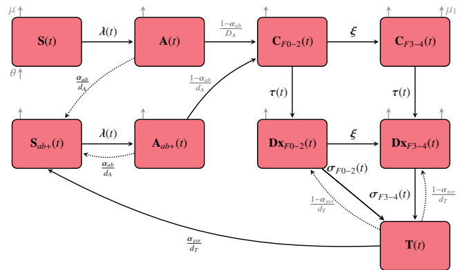
Figure S1.1: Hepatitis C (HCV) natural history and cascade of care. The model is open, and people initiate injection as susceptible ( S(t) ) at a rate \theta . Upon an effective contact, they become acutely infected ( A(t) ) at a time-dependent force of infection \lambda(t) . People spontaneously clear the infection after six months at a probability \alpha_{ab} and become susceptible but antibody positive ( S_{ab+}(t) ). Otherwise, they become chronically infected ( C_{F0-2}(t) ) and progress in fibrosis stages until late HCV infection ( C_{F3-4}(t) ), where they can die of liver-related mortality \mu_1 . Chronically infected people can be diagnosed ( \mathbf{Dx}_{F0-2}(t) , \mathbf{Dx}_{F3-4}(t) ) without regards to disease stage at a rate \tau(t) and then linked to treatment ( \mathbf{Tx}(t) ) at a time varying rate that depends on fibrosis stage ( \sigma_{F0-2}(t) , \sigma_{F3-4}(t) ). Treatment either leads to failure or sustained virologic response and people become susceptible but antibody positive. People who spontaneously cleared or were cured of the disease are susceptible to re-infection with HCV ( A_{ab+} ) at the same force of infection \lambda(t) .
