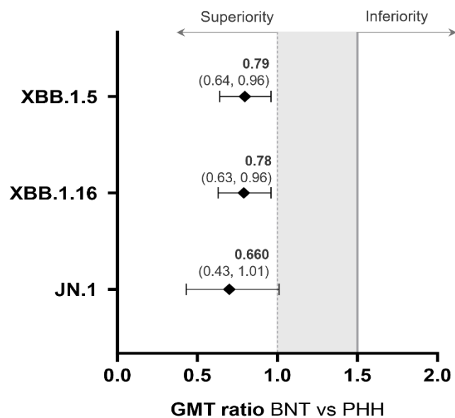
Figure 3. Comparison of the humoral responses elicited by BNT62b2 XBB and PHH-1V81 at Day 14 against SARS-CoV-2 variants Omicron XBB.1.16, Omicron XBB.1.5 and Omicron JN.1
