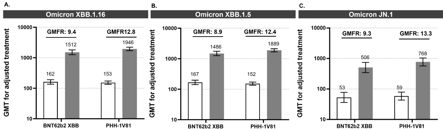
3 A.) GMT for adjusted treatment against Omicron XBB.1.16 variant for each vaccinated group (PHH-1V81 group; n= 406 and BNT62b2 XBB; n=193) by PBNA; (B.) GMT 4 for adjusted treatment against Omicron XBB.1.5 variant for each vaccinated group (PHH-1V81 group; n= 406 and BNT62b2 XBB; n=193) by PBNA; (C.) GMT for adjusted 5 treatment against Omicron JN.1 variant for a subset of n=100 participants (n= 65 with PHH-1V81 and n=35 with BNT62b2 XBB1.5) by VNA. Graphics A-C represent Mean 6 GMT with 95% CI at baseline (with bar) and 14 days after booster (dark grey bar); upper numbers represent mean GMFR at day 14 from baseline. 7 CI: confidence interval; GMT: Geometric Mean Titer; GMFR: Geometric Mean Fold Rise.
