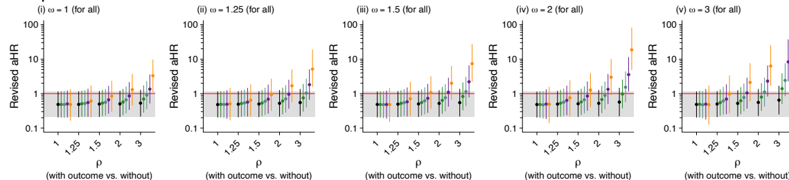
Figure 4: Sensitivity analyses addressing the association of SGTF with risk of emergency department presentation and hospital admission in the presence of differential misclassification of prior infection according to infecting lineage and clinical outcome. We illustrate estimates of the adjusted hazard ratio of progression to (a) emergency department presentation and (b) hospital admission under analyses imputing “full” infection histories for cases under the assumption of differential misclassification of prior infection status. We consider multipliers of 1, 1.25, 1.5, 2, and 3 for the ratio of true to observed infections, first non-differentially among all cases ( \omega ), and for the relative ratio of true to observed infections comparing cases who evaded the indicated outcome versus those who experienced it ( \rho ) and comparing cases infected with BA.2.86-derived lineages to those infected with non-BA.2.86 lineages ( \theta ). Points and lines illustrate median estimates with accompanying 95% confidence intervals. Grey bands illustrate 95% confidence intervals for estimates from the primary analysis.
