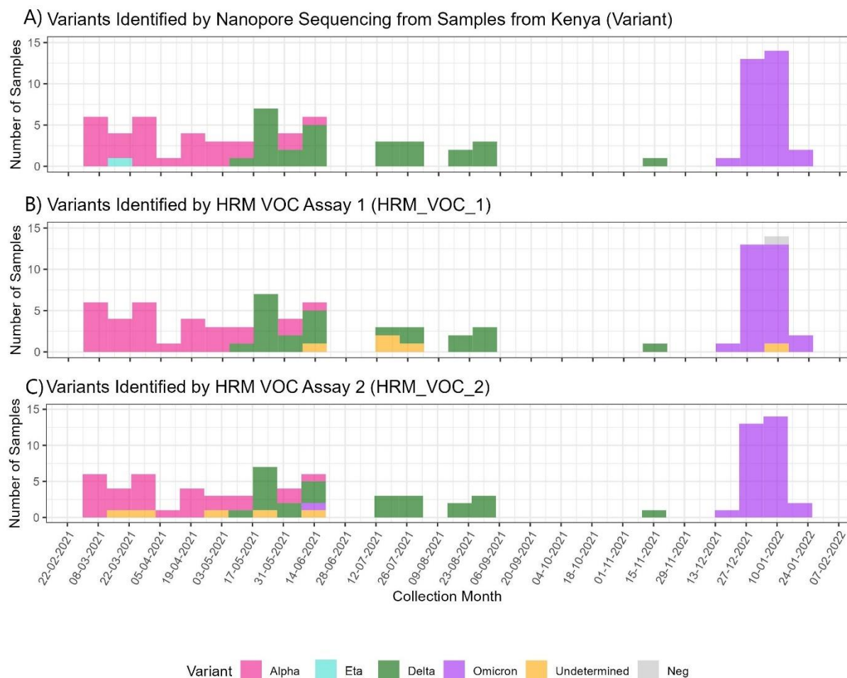
Figure 2 : SARS-CoV-2 Variants identified in Kenya using different methods A) Number of samples collected in Kenya from February 2021 to February 2022 and the variants that were identified by Nanopore Sequencing. B) Number of samples in the Kenyan cohort and the variant identified by using the HRM-VOC-1 assay. Negative results represent those with no amplification observed; undetermined samples had amplification but no identifiable VOC peak. C) Number of samples in the Kenyan cohort and the variant identified using the HRM-VOC-2. Negative results represent those with no amplification observed; undetermined samples had amplification but no identifiable VOC peak.
