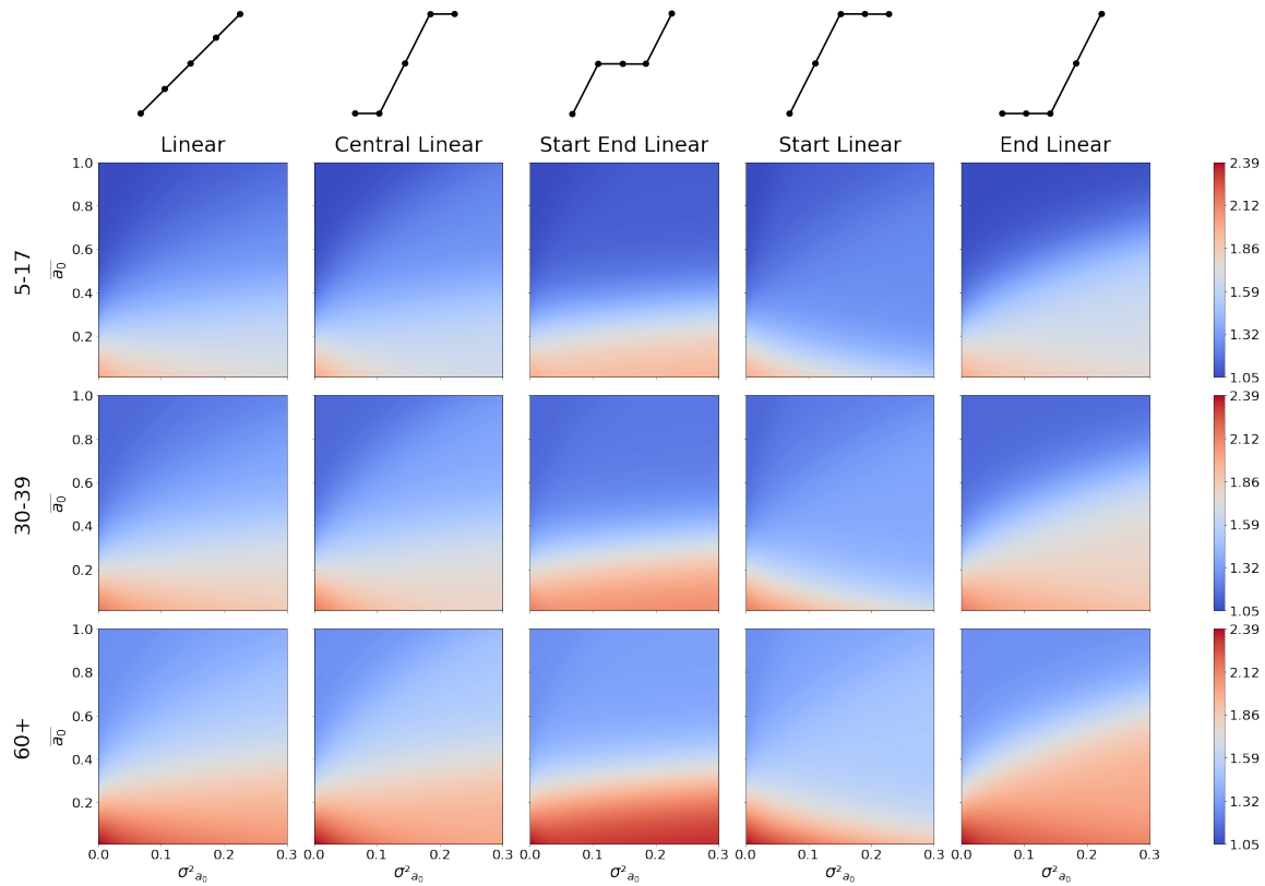
Figure 5: Heatmaps showing the value of R_0 for three age groups (5-17, 30-39, and 60+) as a function of \bar{a}_0 and \sigma_{\bar{a}_0}^2 . Each heatmap refers to one age group (rows) and one of the 5 functions considered (columns). Above each column is a small diagram of the function, showing how the midpoint a_0 varies from small to high perceived severity groups (left to right). The other parameters used for the simulations are \alpha = 10 , \gamma = 5 , \bar{b}_0 = 0.75 , \sigma_{\bar{b}_0}^2 = 0 . We employed a 900-value grid, with 30 values of \bar{a}_0 ranging from 0 to 1, and 30 values of \sigma_{\bar{a}_0}^2 ranging from 0 to 0.3.
