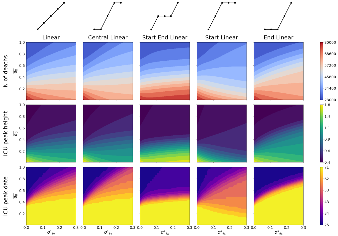
Figure 6: Heatmaps showing the number of deaths (first row), the height of the ICU peak (second row) and its date (third row) as a function of \bar{a}_0 and \sigma_{a_0}^2 . Each column corresponds to one of the five functions linking perceived severity and midpoint of the logistic curve giving the transition rate from compliant to non-compliant compartments as a function of the fraction of vaccinated individuals. Above each column is a small diagram of the function, showing how the midpoint a_0 varies, going from small to high perceived severity groups (left to right). The other parameters used for the simulations are \alpha = 10 , \gamma = 5 , \bar{b}_0 = 0.75 , \sigma_{b_0}^2 = 0 . We employed a 900-value grid, with 30 values of \bar{a}_0 ranging from 0 to 1, and 30 values of \sigma_{a_0}^2 ranging from 0 to 0.3. The rugged profile of the curves related to the peak date is due to its discrete nature, with values representing the (integer) number of days after the simulation's start in which the peak is observed.
