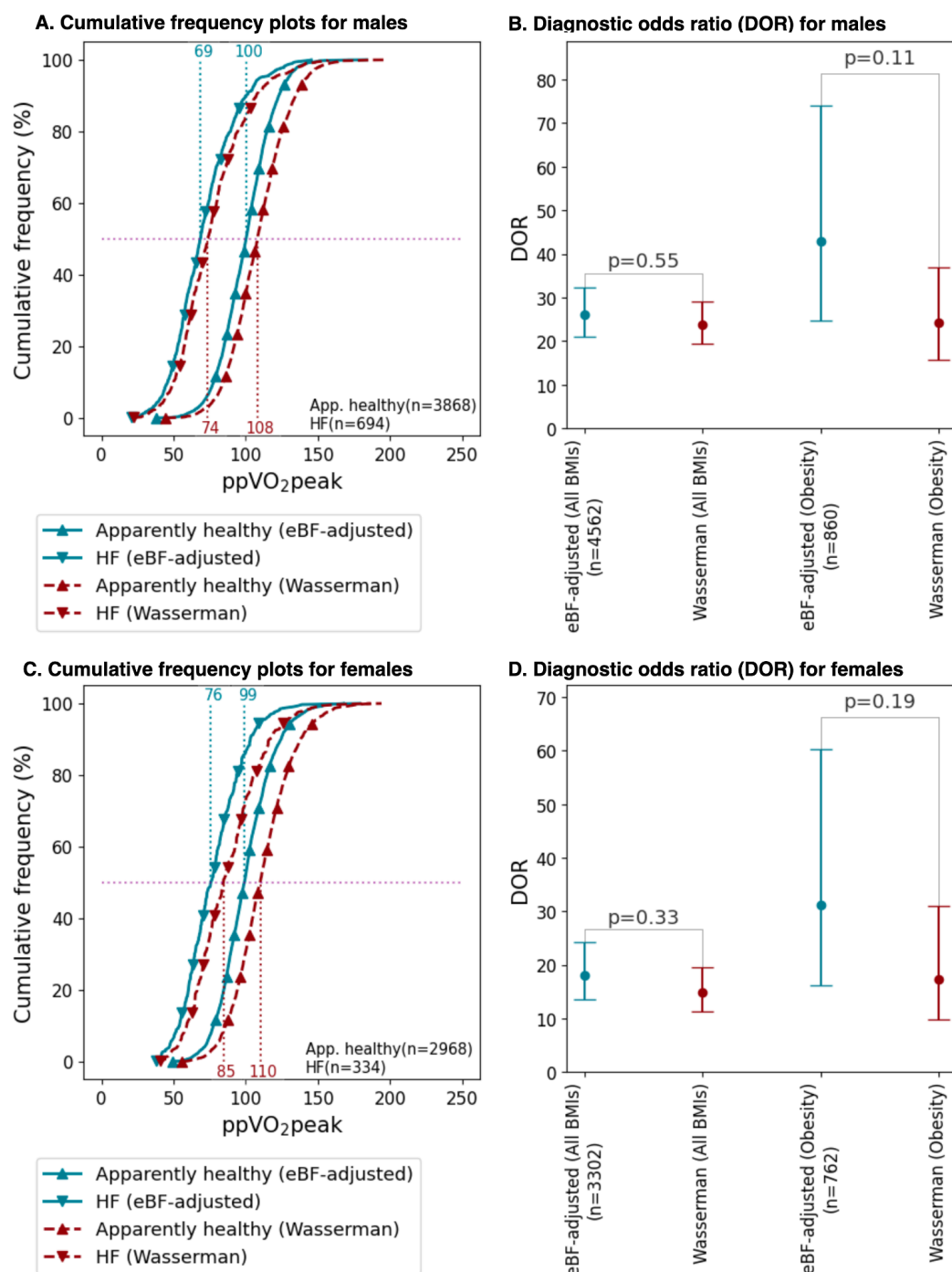
Figure 6. Application of novel eBF-adjusted VO_2 peak equation in diagnosing heart failure (HF), as compared to the Wasserman equation.
