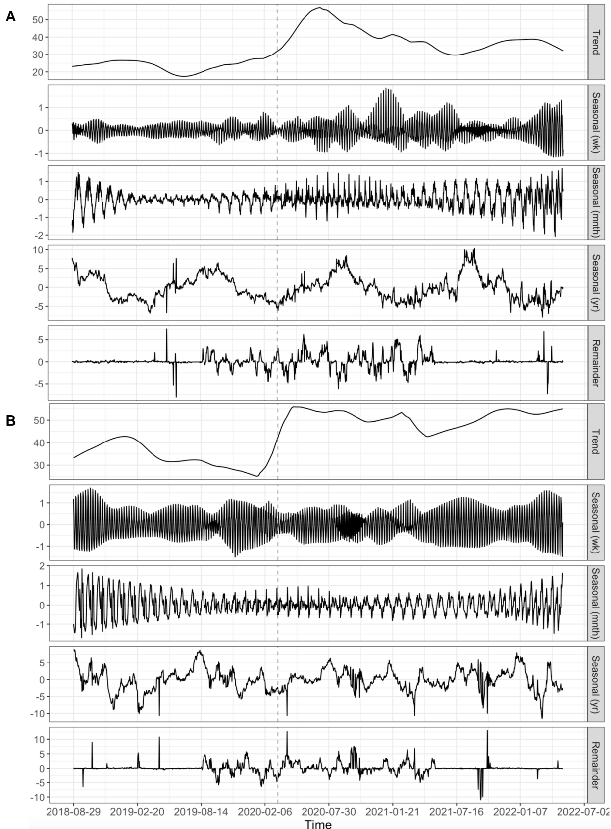
Figure 5. MSTL Models
