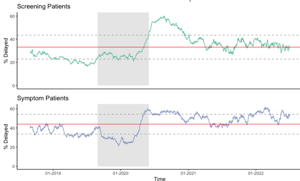
Figure 4. SARIMAX Models.
