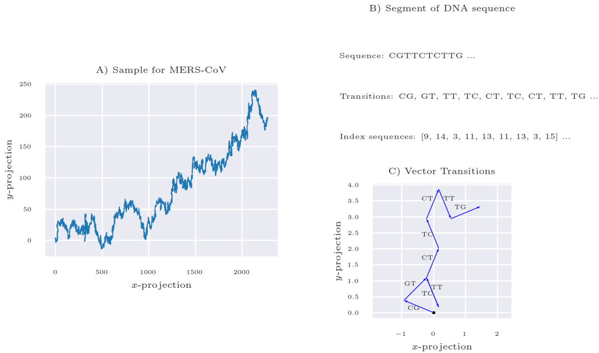
Figure 3: Transformation of DNA sequences into 2D vector transitions. Panel A presents a complete DNA sequence of a virus, dynamically unfolded in a two-dimensional continuum, revealing intricate patterns and relational nuances inherent in the sequence. Panel B focuses on a segment of the DNA sequence, disclosing individual base transitions and their corresponding sequential indices, elucidating the core mechanics of our encoding strategy. Panel C showcases the conversion of a DNA sequence segment into expressive vectors in the two-dimensional domain, highlighting the innovative transformation process that simplifies the visualization and analysis of complex genetic data.
