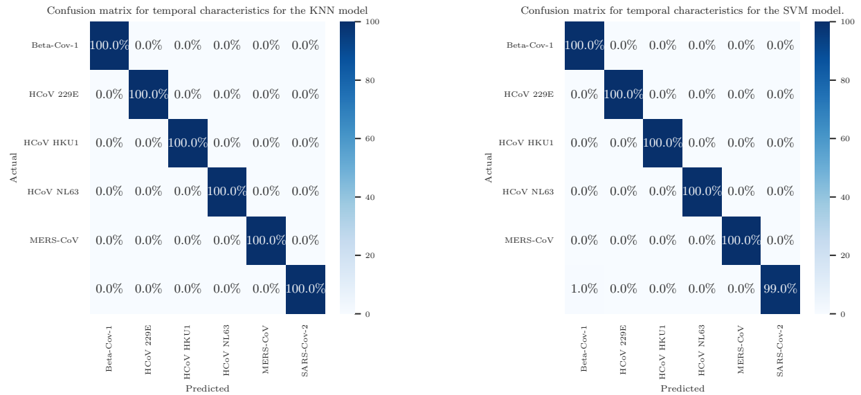
(c) Confusion matrix referring to test data from the KNN model for the six predicted classes.
