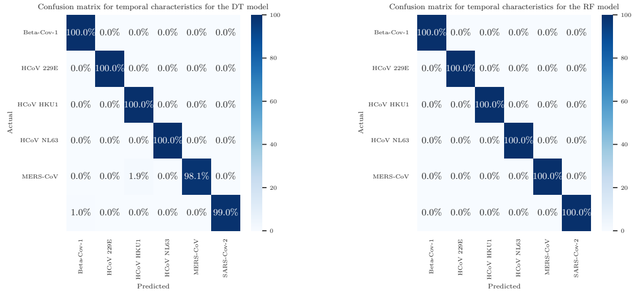
(a) Confusion matrix referring to test data from the DT model for the six predicted classes.
