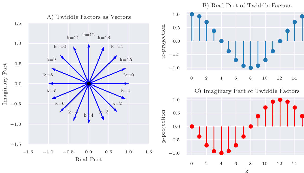
Figure 2: Visualization of Twiddle Factors encoding transitions between nucleotide bases. Pannel A) visually represents twiddle factors as vectors within the complex plane, with annotations denoting their respective values of k . Pannels B) and C) display the real and imaginary components of the twiddle factors, respectively.
