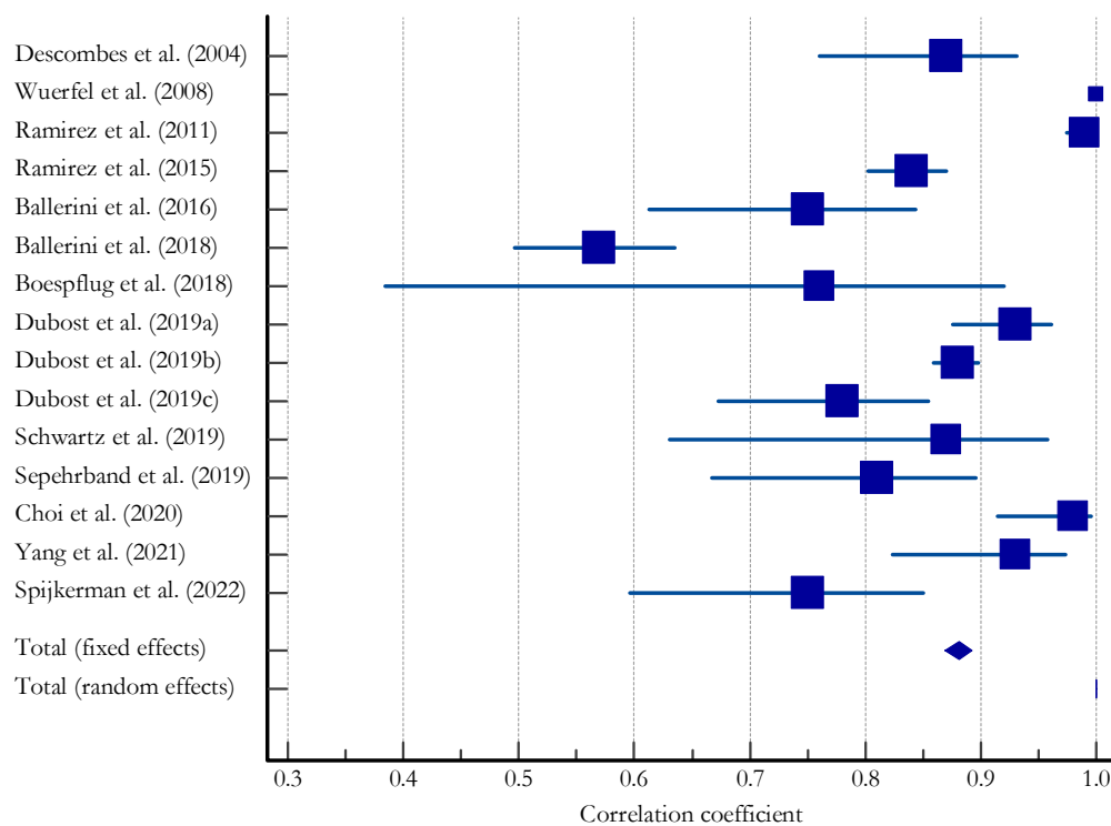
Figure 4. Forest plot of correlation coefficients of best performance (non-computational vs. computational) PVS quantification (MedCalc ( https://www.medcalc.org/ )). Square size indicates relative sample size, diamond indicates pooled fixed and random effects correlation coefficient.
