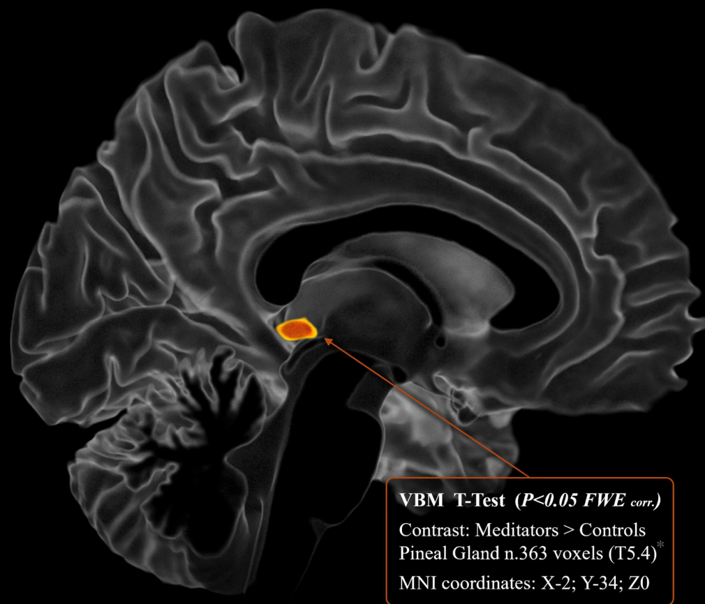
Descriptives - Pineal Gland
