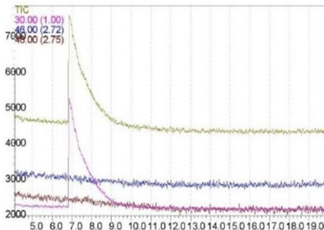
Figure 1. Select Ions Monitoring (SIM) Chromatograms for NO (30), NO 2 (46), O 3 (48) and the Total Ion Chromatogram (TIC) from a PDEB™ Output Stream Gas Aliquot.
