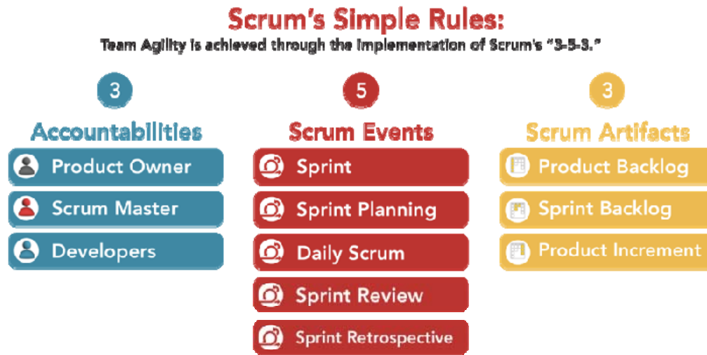
Figure 1. Scrum Implementation
