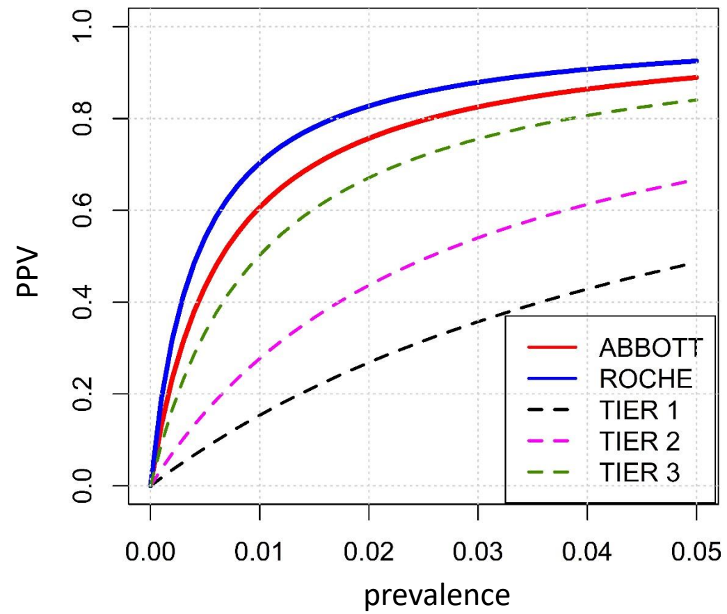
PPV vs. prevalence
