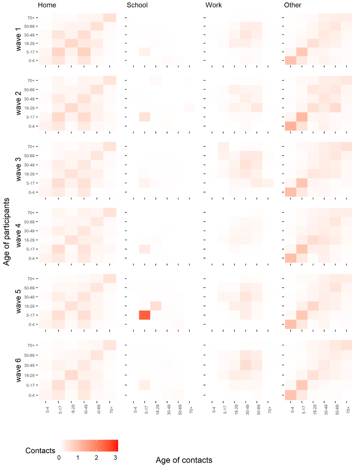
Fig 4: Imputed setting-specific social contact matrices showing mean number of daily contacts for the six waves in the CoMix survey. Locations include all contacts made in the home, at schools, at workplaces and other community contacts (transport, sport activities etc.). Note that some contacts overlap as multiple settings could be registered for the same contact. The matrices represent bootstrap mean values of N=10 000 samples. Data were weighted on age and adjusted for reciprocity of contacts.
