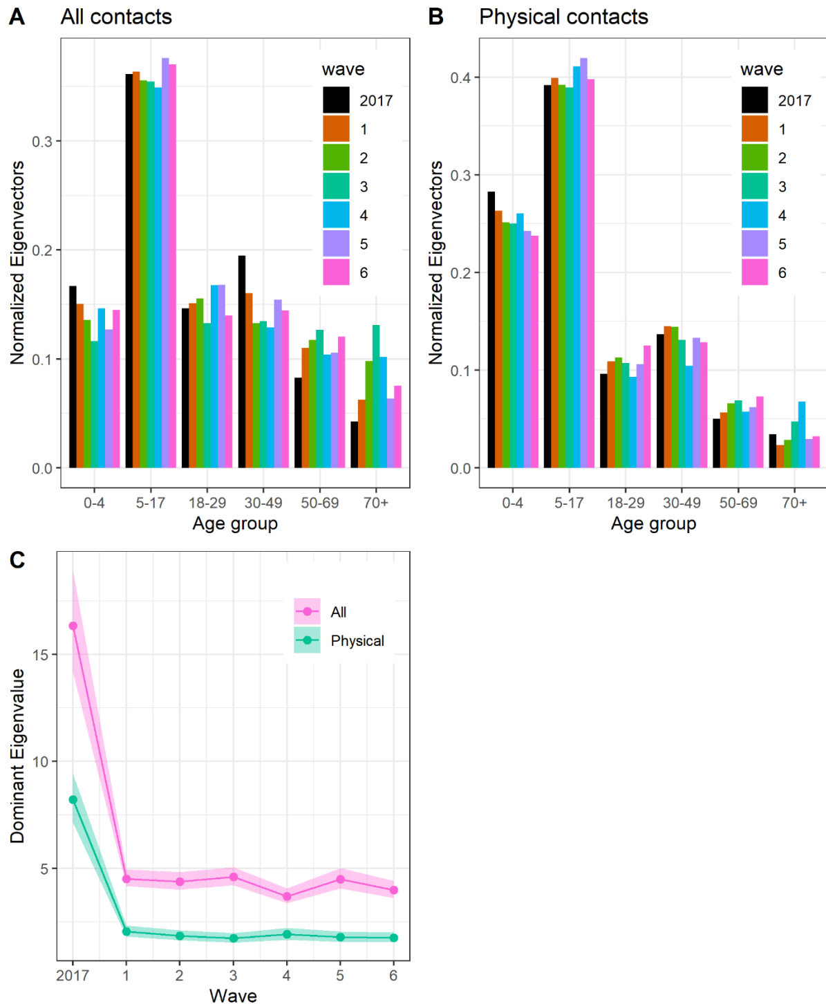
Fig 5: Comparison of CoMix and baseline dominant eigenvectors and eigenvalues: (A) Dominant normalised eigenvectors from contact matrices of all contacts by age group, (B) Dominant normalised eigenvectors from contact matrices of physical contacts by age group, (C) dominant (maximum) eigenvalues of contact matrices for all contacts (red) and physical contacts (green).
