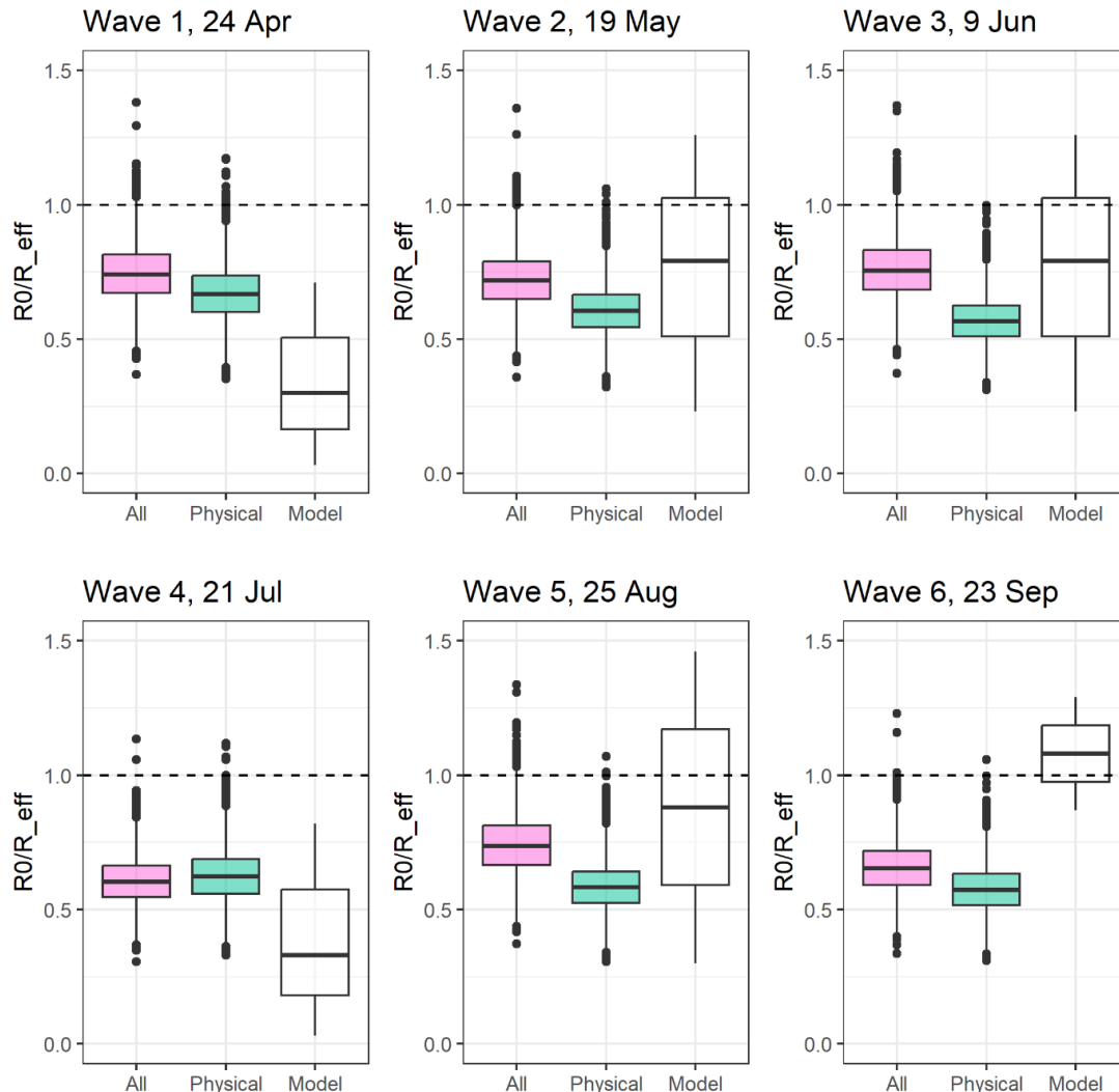
Fig 6: Boxplot showing estimated R0 reproduction numbers for the CoMix waves (all contact matrices and physical contact matrices), multiplying maximum eigenvalue ratios (Imp CoMix/Baseline) from imputed contact matrices with R0 from a calibrated mathematical model prior to the lockdown in Norway (10, 22). For comparison is shown the estimated effective reproduction numbers R_e(t) from the same model during the waves
