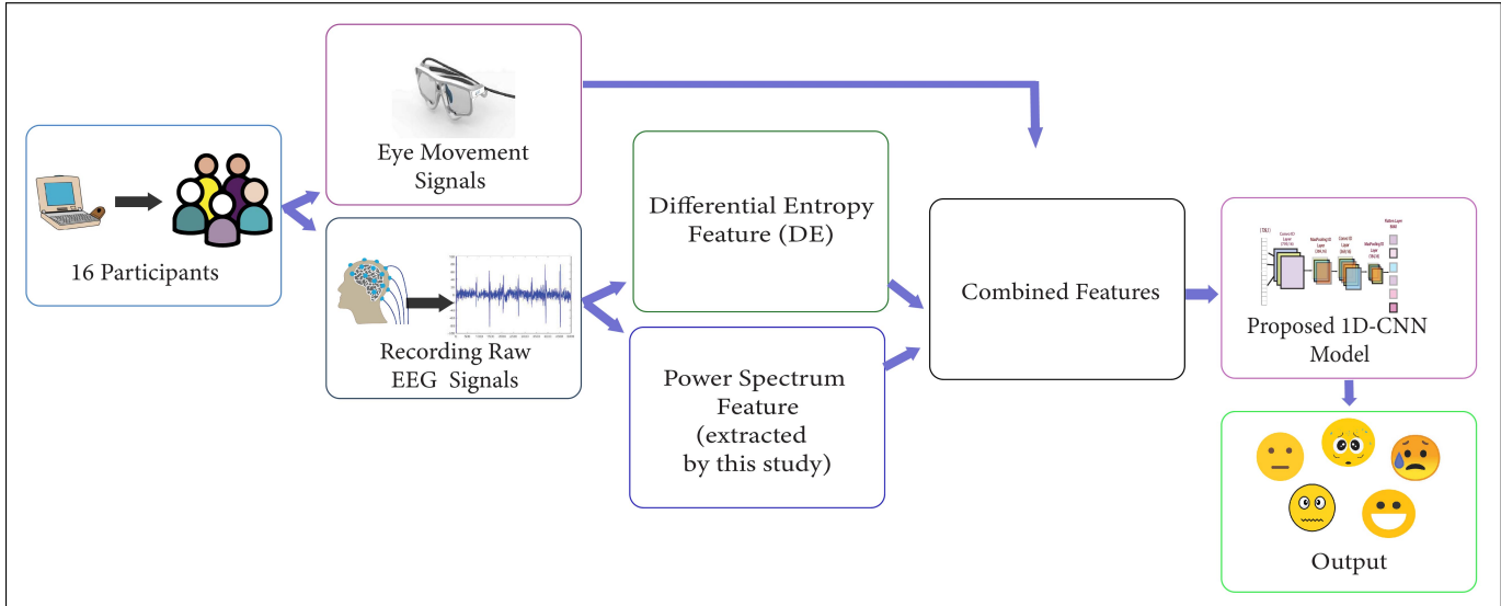
Fig. 1. Complete workflow of the proposed system on the SEED-V dataset.
