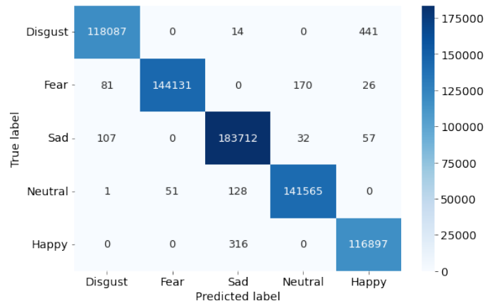
Fig. 5. Confusion matrix
