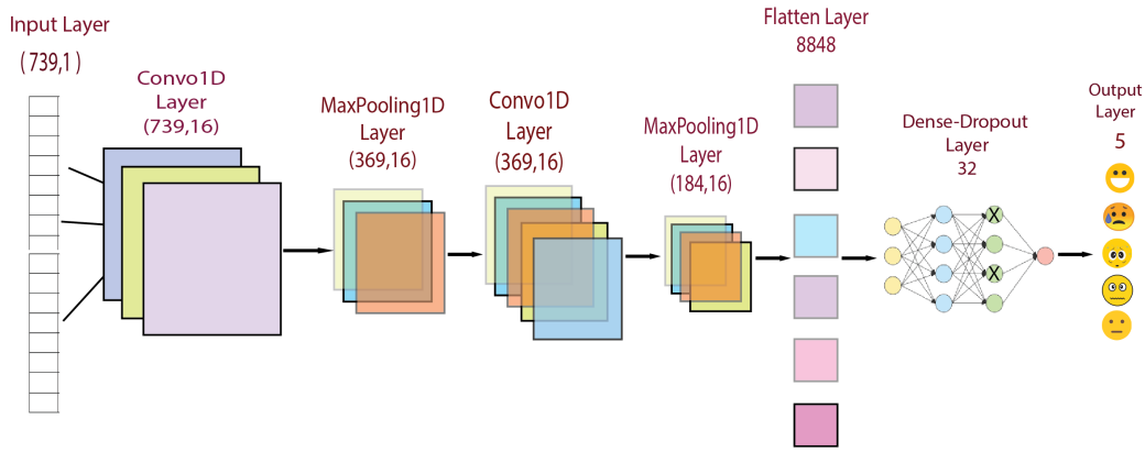
Fig. 4. Our proposed 1D-CNN model architecture
