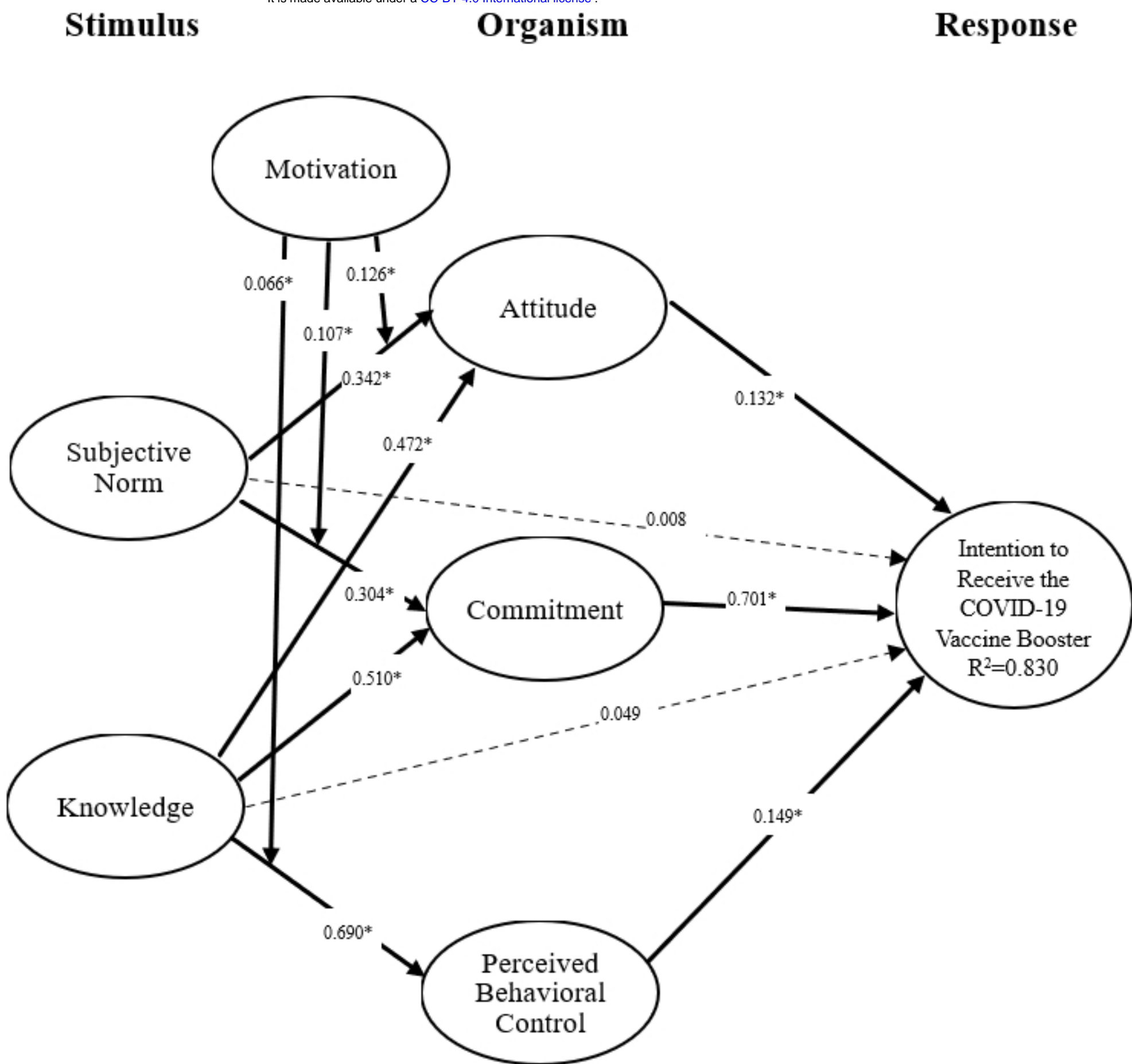
Figure 2. The results of integrating SOP and TPB model
