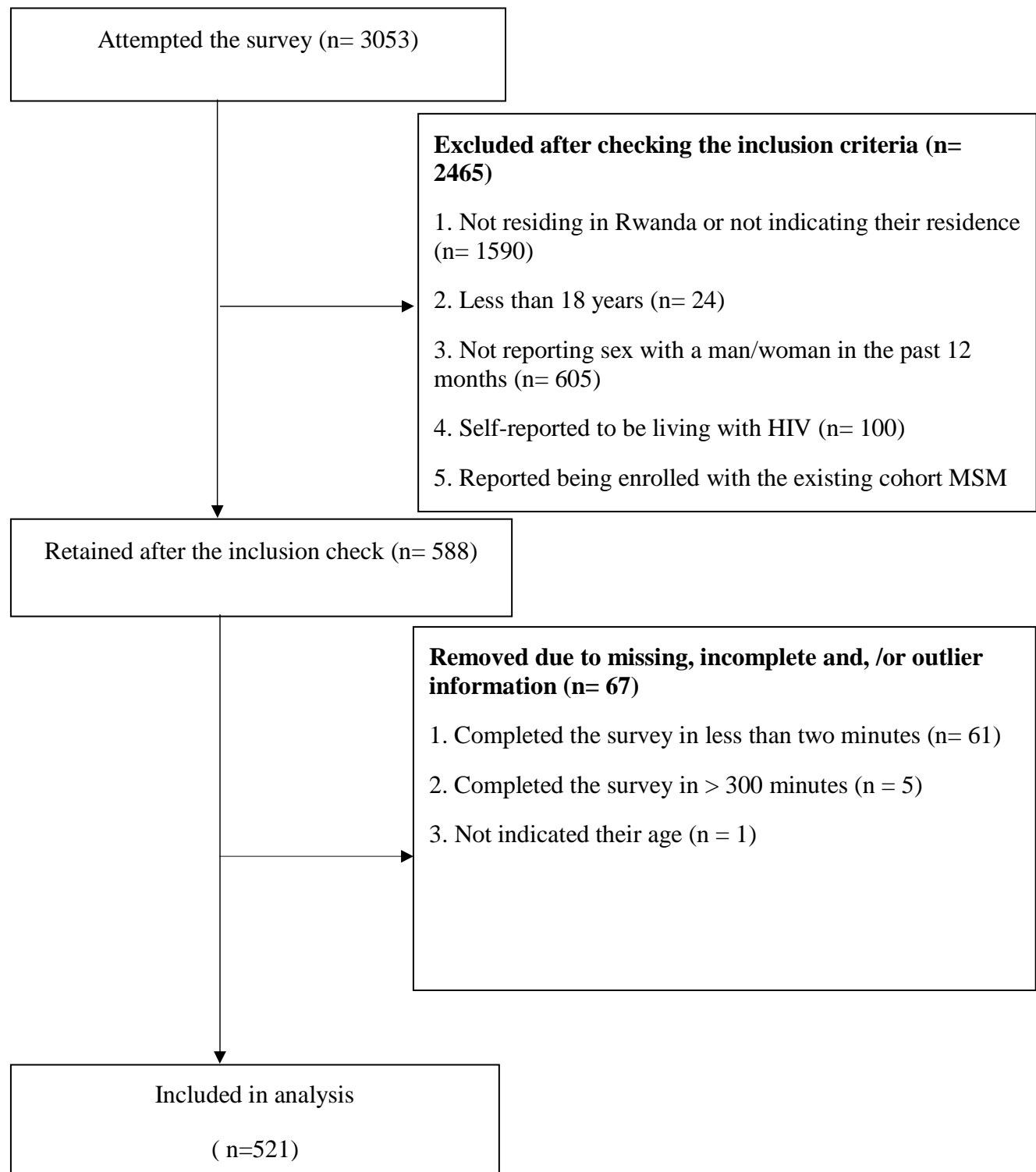
Figure 2. Data flow
