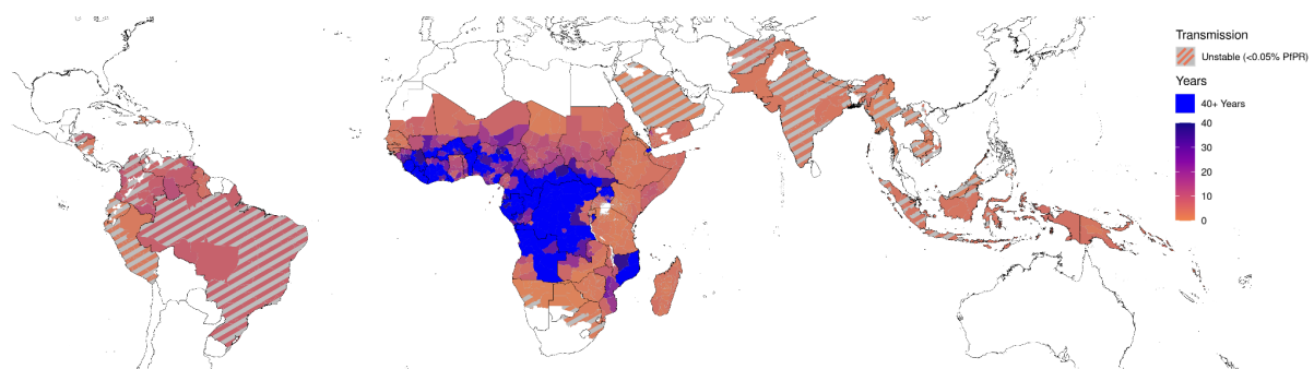
Figure 3. Global distribution of predicted times for the percentage of clinically relevant infections misdiagnosed due to pfhrp2/3 gene deletions to increase from 1% to 5%. Regions estimated not to reach 5% within 40 years are shown in blue. Regions with very low, unstable malaria transmission (defined as <0.05% malaria prevalence) are shown with diagonal grey lines. (See Supplementary Figure 9 for focus on Africa).
