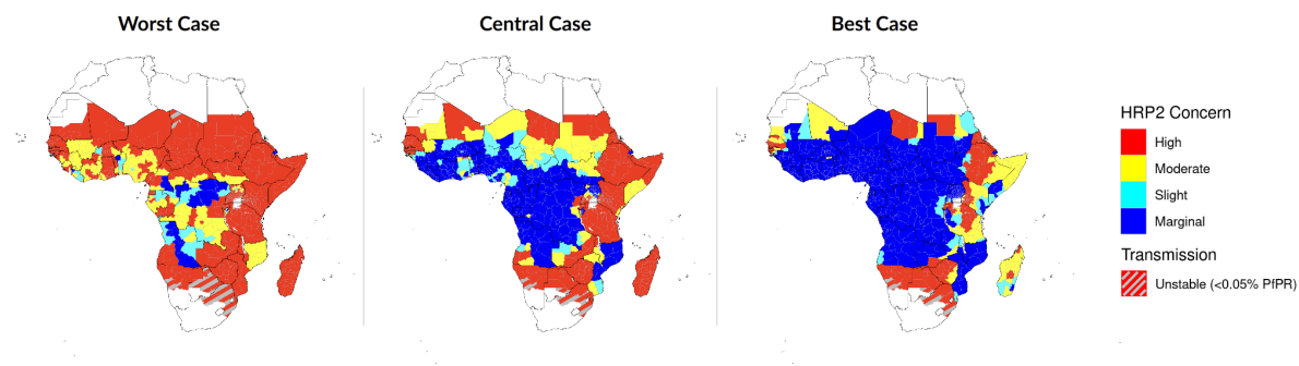
Figure 4. Innate risk score for the concern caused by pfhrp2 deletions in Africa. High (red), moderate (yellow) and slight (teal) risk represent >5% of clinically relevant infections misdiagnosed due to pfhrp2/3 gene deletions in less than 6, 12 and 20 years respectively, and marginal risk (blue) represents <5% in 20 years. Uncertainty in model parameters for each region impacts risk scores, with the worst and best case scenarios (based on the uncertainty in the range of parameters explored) shown. Regions with very low, unstable malaria transmission (defined as <0.05% malaria prevalence) are shown with diagonal grey lines. (See Supplementary Figure 10 for global risk scores).
