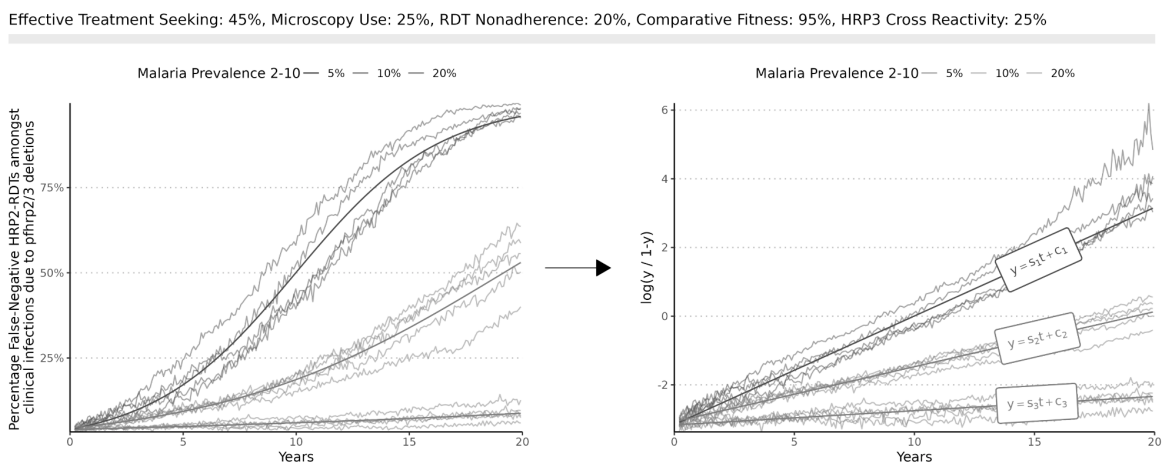
Figure 1. Conversion from model simulations to selection coefficients. For a given parameter set (effective treatment-seeking: 45%, microscopy use: 25%, RDT nonadherence: 20%, comparative fitness: 95%, HRP3 cross reactivity: 25%), the simulated percentage of false-negative HRP2-based RDTs amongst clinical infections due to pfhrp2/3 deletions ( y ) is converted to log odds ( y/(1-y) ), with the gradient calculated to estimate the selection coefficient.
