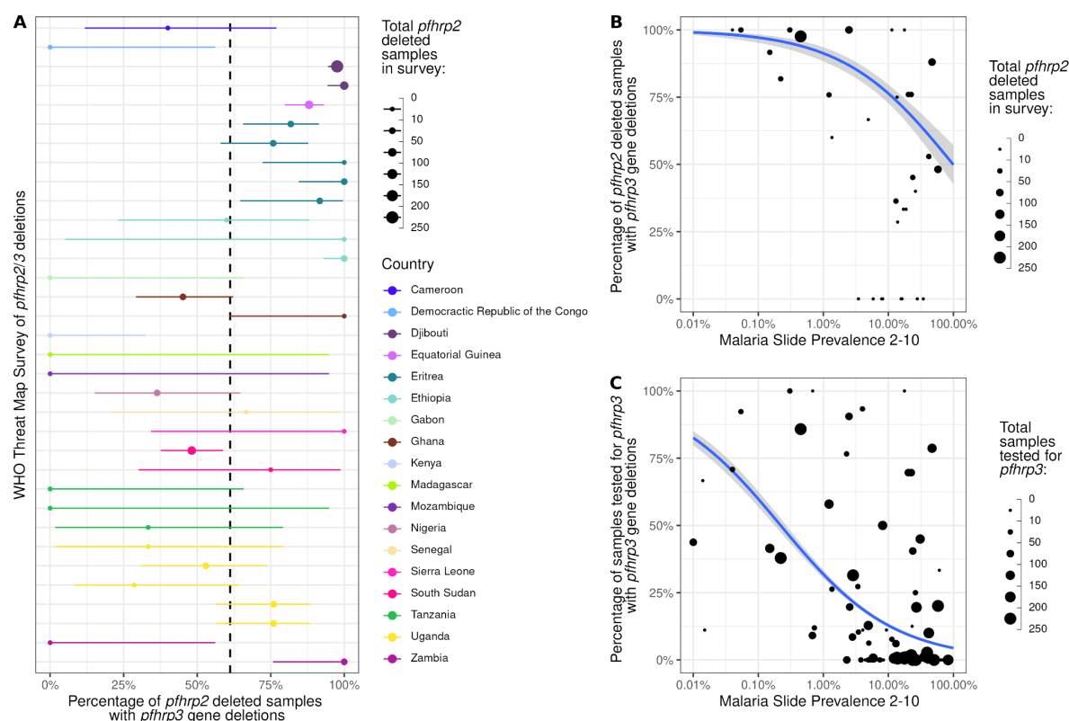
Figure 2. Distribution and independence of pfhrp2/3 deletions in Africa collated in the WHO Malaria Threat Maps database. A) Percentage of pfhrp2 -deleted samples also with pfhrp3 deletions by survey. The mean and 95% confidence interval is shown with points and ranges. B). Relationship between the percentage of pfhrp2 -deleted samples with pfhrp3 deletions and malaria slide prevalence in 2-10 year-olds based on Malaria Atlas Project estimates. Binomial regression model fit (blue) shows the mean relationship between malaria prevalence and pfhrp2 deletion frequency among pfhrp3 -deleted parasites, with the 95% confidence interval of the regression fit shown with shaded bands. C). Relationship between the percentage of samples with pfhrp3 deletions and malaria prevalence. In all plots, the point size represents the number of samples from each survey used to derive estimates.
