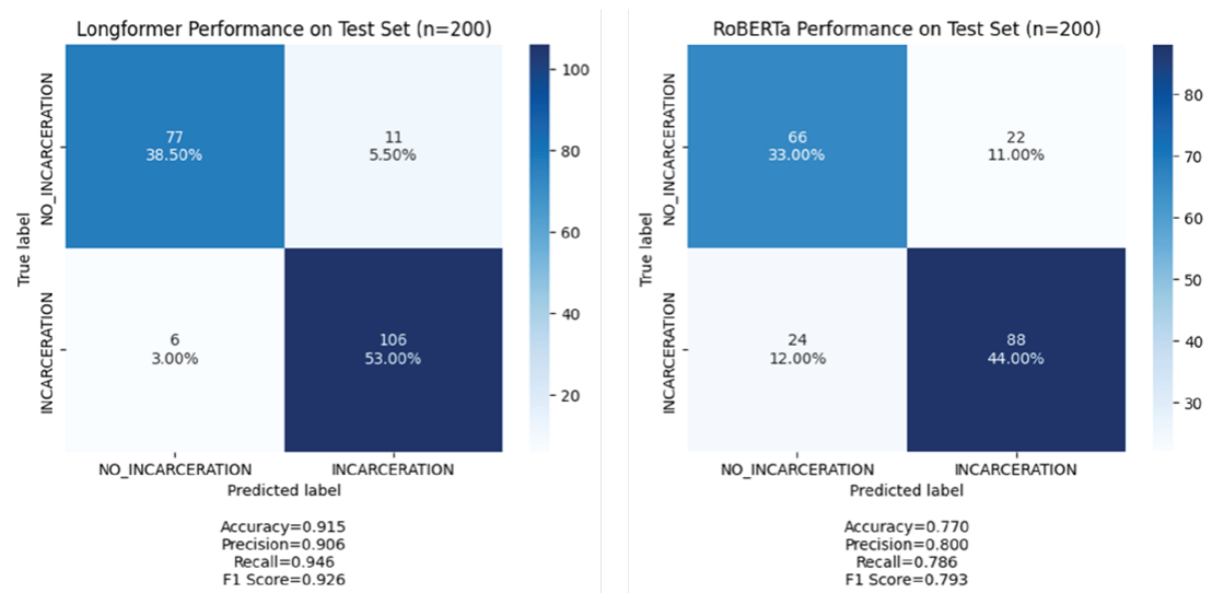
Figure 2. Longformer and RoBERTa Predicted Label vs. True Label by Manual Annotation
