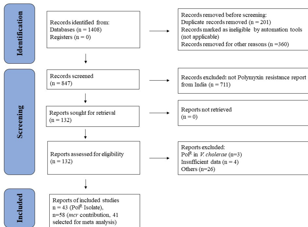
334 Figure 1. The PRISMA flow diagram for the selection, inclusion, and exclusion of studies.
