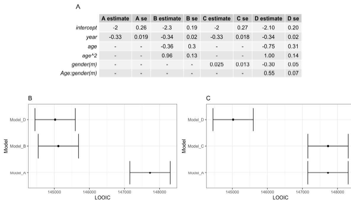
Figure 14: Philosophical sensitivity analysis. A) Comparison of posterior parameter values across models. B) LOOIC for nested models with age. C) LOOIC for nested models with gender.
