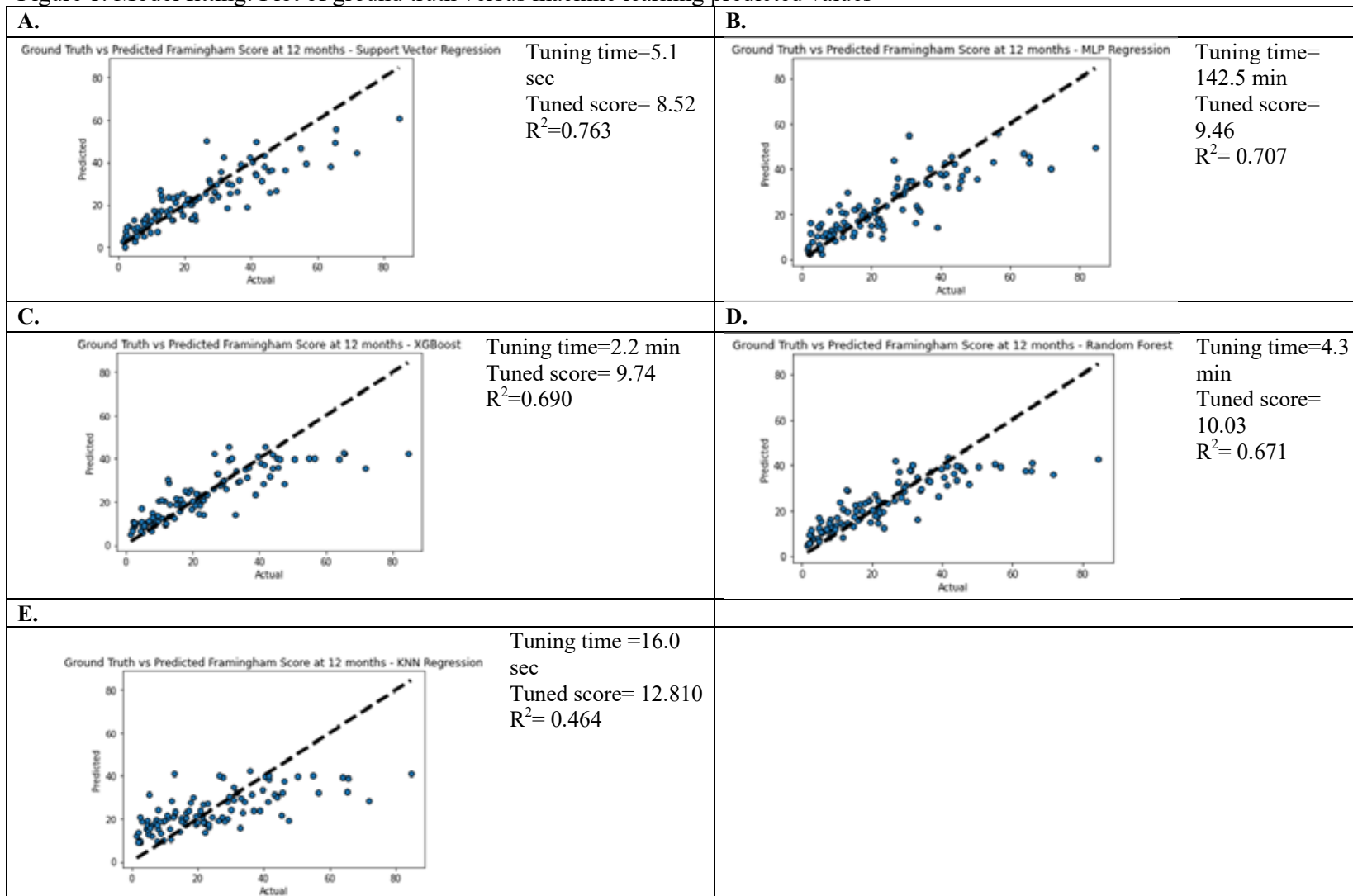
Figure 1: Plot of ground truth versus machine learning predicted values. The tuning time to optimise each machine learning method is shown on the panel. It was longest for multilayer perceptron (MLP) and shortest for support vector regression (SVR). There was deviation of the predicted from
