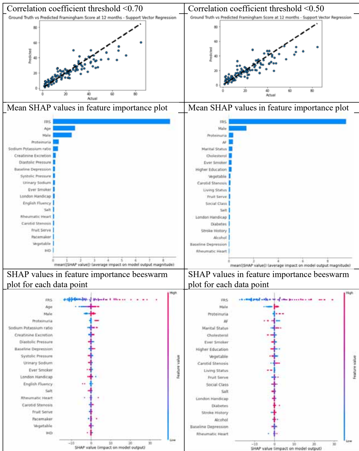
Figure 3: The R^2 drops from 0.770 for 32 variables data with down to 0.728 with 23 variables. FRS, Framingham risk score; IHD, ischemic heart disease, AF, atrial fibrillation; HbA1c, glycosylated hemoglobin.
