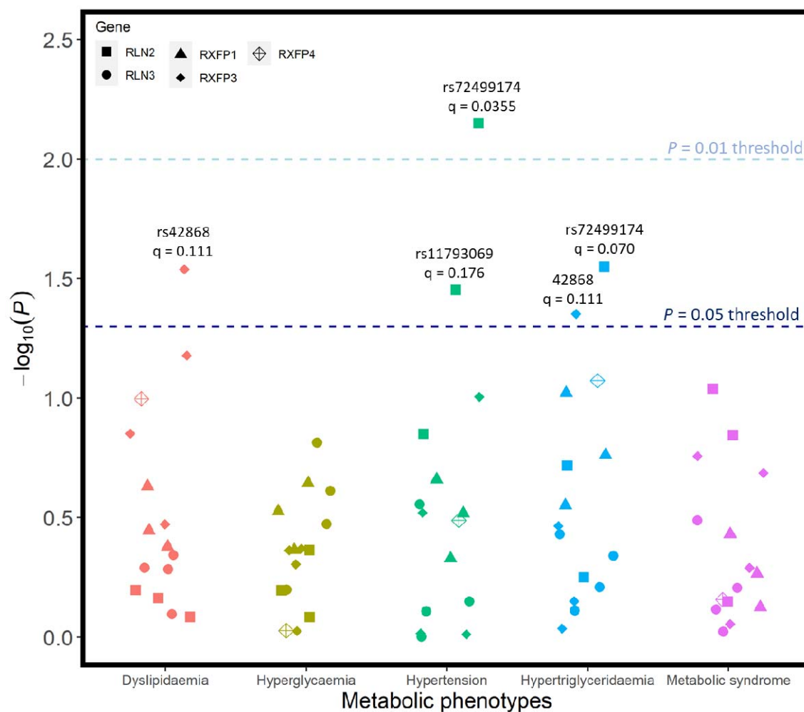
Figure 5: Unadjusted p-values for association tests between all SNPs and metabolic syndrome, as well as 4 sub-outcomes that comprise metabolic syndrome. Regression models were adjusted for age, age 2 , sex, genotyping batch, testing centre, and the first six European ancestry principal components. SNPs that were nominally associated with a phenotype are annotated with their corresponding q-value following FDR correction – there were no statistically significant associations.
