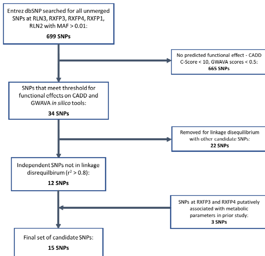
Figure 1: Flowchart outlining the process used to select candidate single nucleotide polymorphisms in this study.
