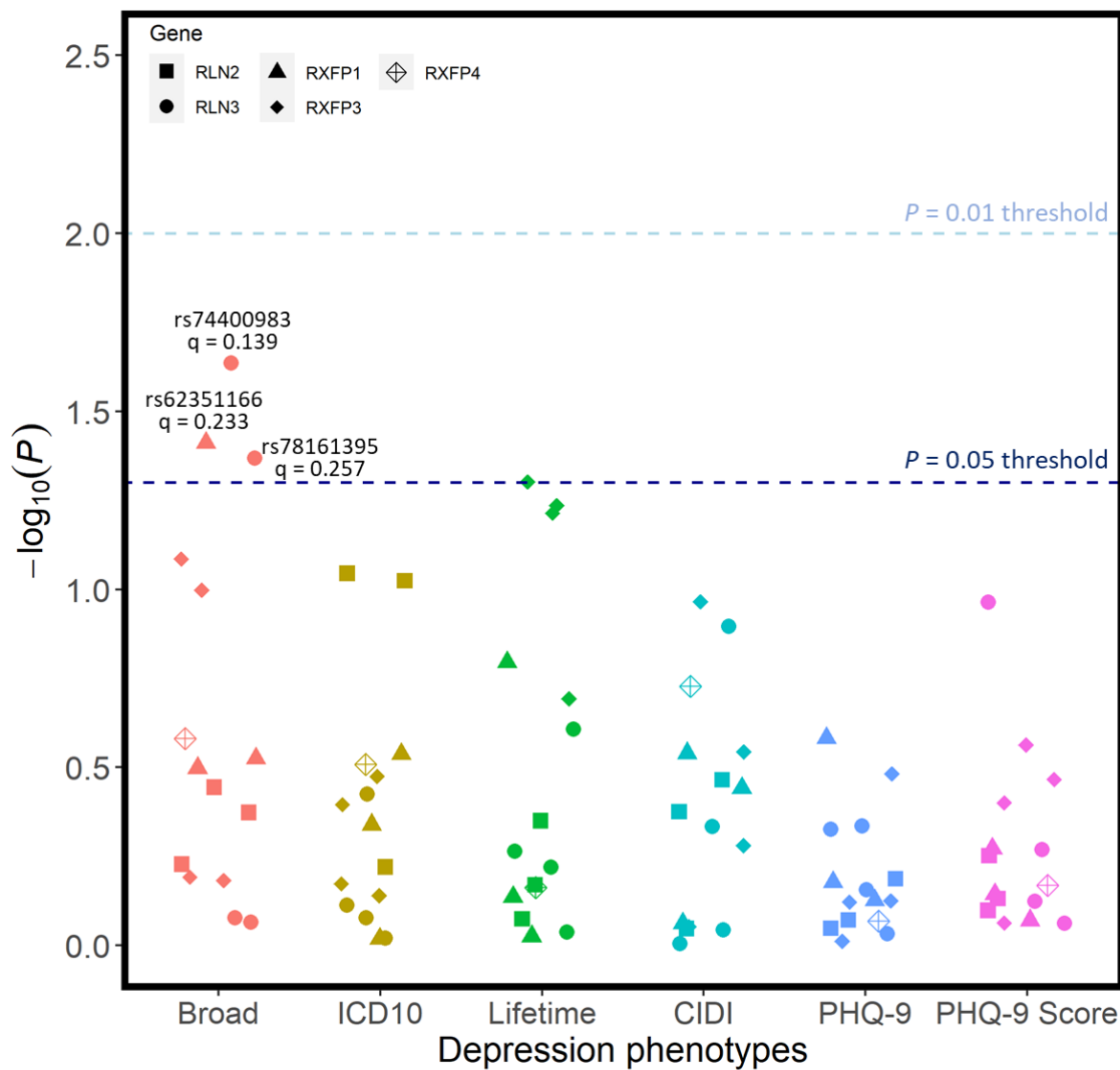
Figure 2: Unadjusted p-values for association tests between all SNPs and the 6 phenotypic definitions of depression. Regression models were adjusted for age, age 2 , sex, genotyping batch, testing centre, and the first six European ancestry principal components. SNPs that were nominally associated with a phenotype are annotated with their corresponding q-value following FDR correction – there were no statistically significant associations.
