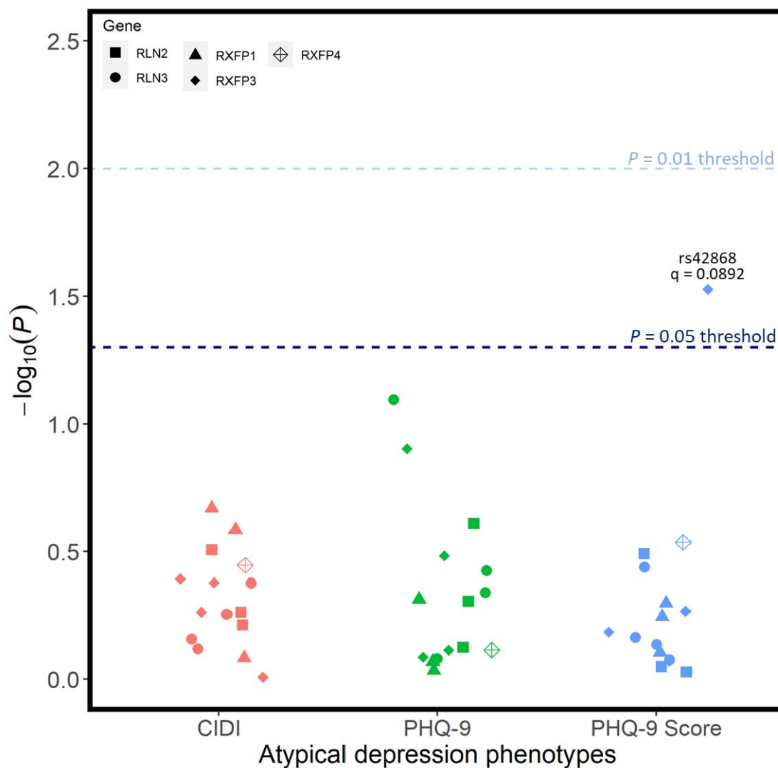
Figure 3: Unadjusted p-values for association tests between all SNPs and the 3 phenotypic definitions of atypical depression. Regression models were adjusted for age, age 2 , sex, genotyping batch, testing centre, and the first six European ancestry principal components. SNPs that were nominally associated with a phenotype are annotated with their corresponding q-value following FDR correction – there were no statistically significant associations.
