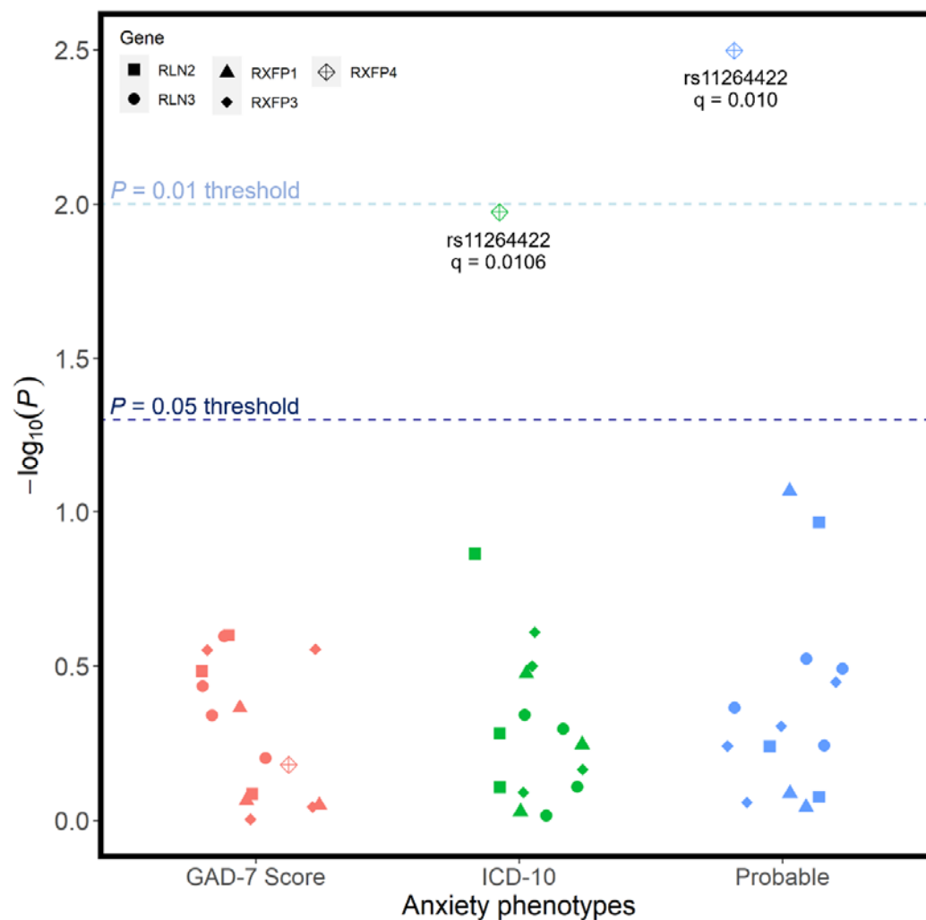
Figure 4: Unadjusted p-values for association tests between all SNPs and the 3 phenotypic definitions of anxiety disorders. Regression models were adjusted for age, age 2 , sex, genotyping batch, testing centre, and the first six European ancestry principal components. SNPs that were nominally associated with a phenotype are annotated with their corresponding q-value following FDR correction – there were no statistically significant associations.
