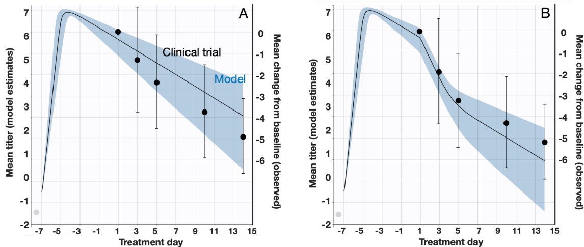
Fig. 1. Estimated and observed viral load following treatment with (A) placebo or (B) Paxlovid. The left y-axes, black lines, and blue shading indicate the means and 95% confidence intervals of SARS-CoV-2 viral load (RNA log 10 copies/mL) as estimated by the fitted within-host model. The right y-axes, black dots and error bars indicate the means and 95% confidence intervals of the decrease in viral load since the initiation of treatment as reported in a clinical trial in which 1126 COVID-19 patients received a placebo and 1120 patients received Paxlovid between July 16 and December 9, 2021 (16). Day one corresponds to the initiation of treatment. The gray circles denote the assumed initial viral load upon infection ( V_0 ) corresponding to one infectious virus particle in the upper respiratory tract (24).
