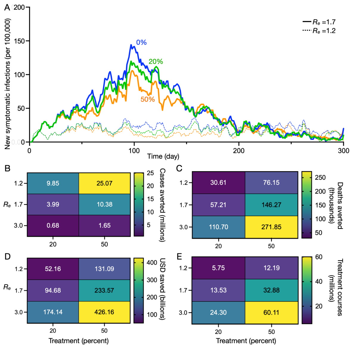
Fig. 2. Projected health and economic impacts of a large-scale SARS-CoV-2 antiviral campaign over 300 days in the US, across a range of transmission and treatment scenarios. (A) Estimated incidence of symptomatic SARS-CoV-2 infections across three treating scenarios: 0%, 20%, or 50% of symptomatic cases receive a five-day Paxlovid regimen started within three days of symptom onset (indicated by line color). Dashed and solid curves correspond to effective reproduction numbers of 1.2 and 1.7, respectively. The four heat maps provide estimates across three different effective reproduction numbers (rows) and two different treatment rates (columns), of the following quantities: (B) number of cases averted (millions), (C) number of
