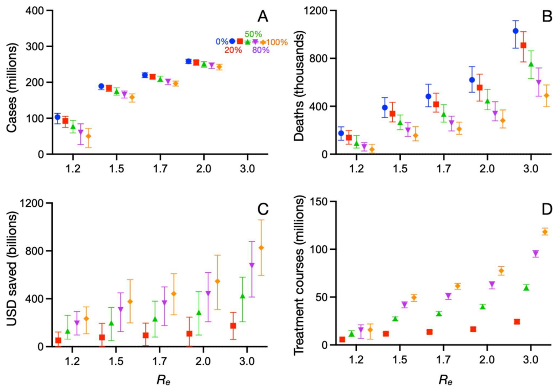
Fig. 3. Projected health and economic impacts of a large-scale SARS-CoV-2 antiviral campaign over 300 days in the US, across a range of transmission and treatment scenarios.
