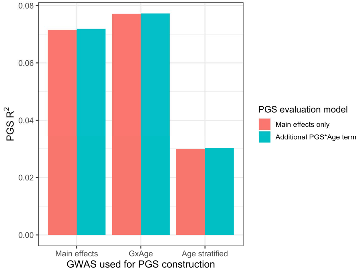
Figure 7. PGS R 2 based on three sets of GWAS setups. “Main effects” were from a typical main effect GWAS, “GxAge” effects were from a GWAS with a SNP-age interaction term, and “Age stratified” GWAS had main effects only but were conducted in four age quartiles. PGS R 2 was evaluated using two models: one with main effects only, and one with an additional PGS*Age interaction term.
