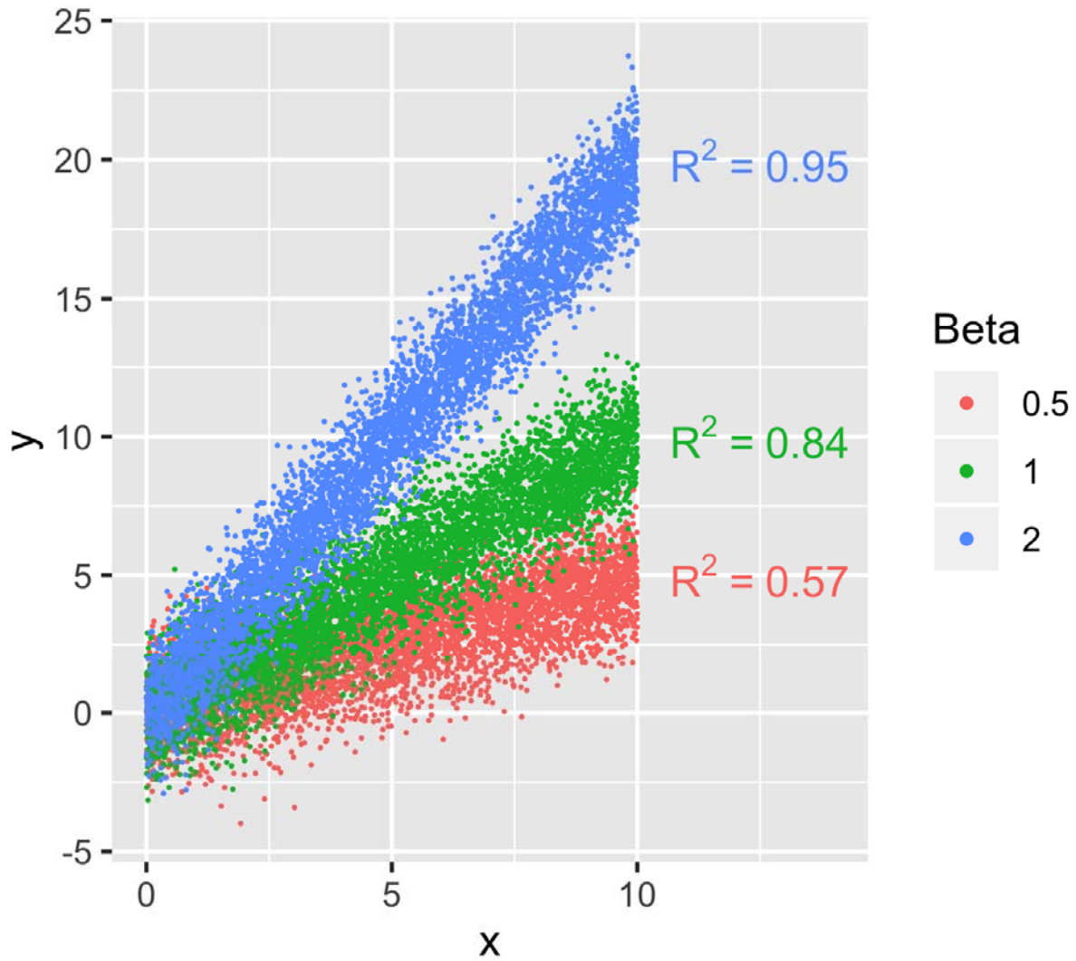
924 S Figure 2. Three sets of simulated data with varying regression line slopes, showing how model 925 R^2 changes when regression line slope changes, all else being equal. Residuals were sampled 926 from a normal distribution (mean=0, sigma= \sqrt{\pi/2} ) to give mean squared error=1. 5,000 x- 927 values were sampled for each line, uniformly distributed from 0-10. Despite having the same 928 mean squared error, model R^2 increases as beta increases. 929 930
