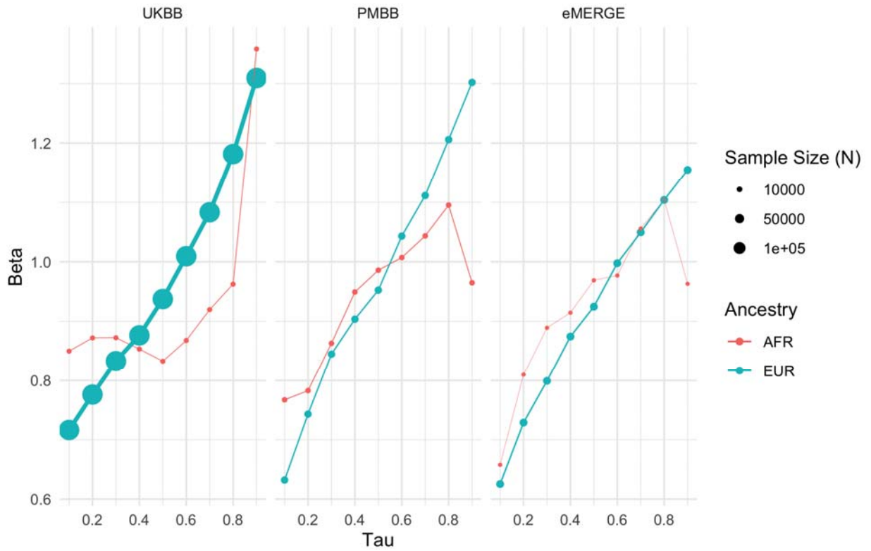
Figure 5. Quantile regression effects of PGS BMI (in units of log(BMI)) on log(BMI) at each decile of BMI in each cohort and ancestry. The effect of PGS BMI increases as BMI itself increases, suggesting that no individual covariate-PGS interaction is responsible for the nonlinear effect of PGS BMI .
