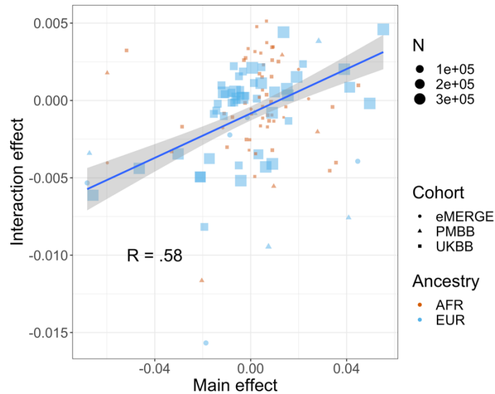
Figure 4. Relationships (Pearson correlations weighted by sample size) between maximum R^2 differences across strata, main effects of covariate on \log(\text{BMI}) , and PGS-covariate interaction effects on \log(\text{BMI}) . Main effect units are in standard deviations, interaction effect units are in PGS standard deviations multiplied by covariate standard deviations. Only continuous variables are plotted and modeled. GERA was excluded due to slightly different phenotype definitions.
