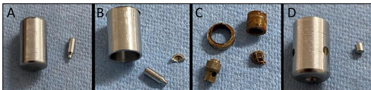
278 279 Figure 5: Photographic images of the nozzle parts after exposure to the cytostatic solution. Nozzle A, 280 B, C, D.
