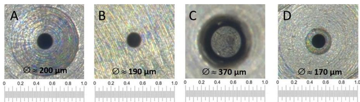
211 Figure 2: Light microscopic images of the outlet orifices with determined orifice diameters of the 212 examined nozzles; scaling in mm. Nozzles A, B, C, D
