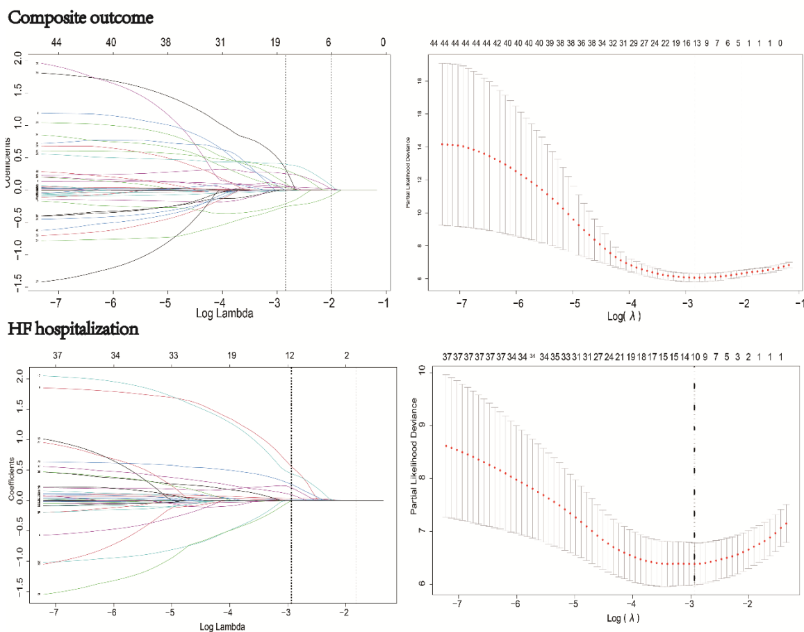
Figure S2:LASSO Regression analysis
