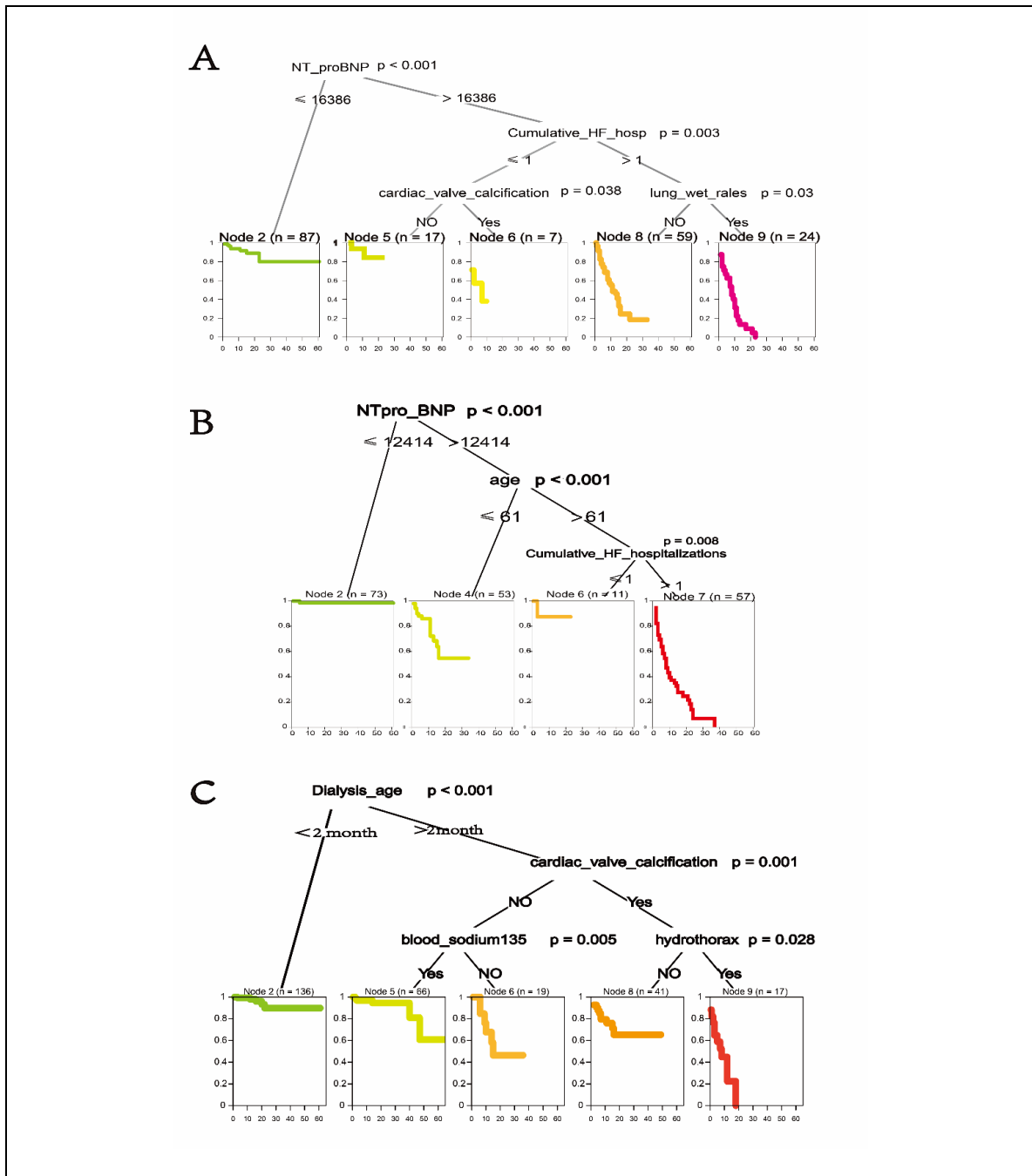
Figure 5 (A) composite outcome prediction model; (B) heart failure hospitalization prediction model; (C) death prediction model
