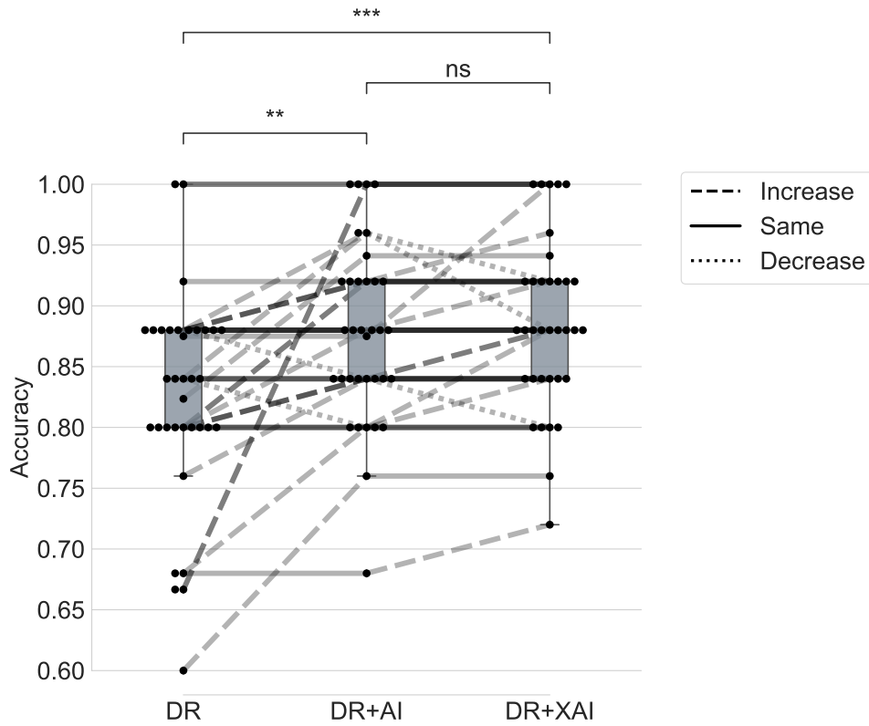
Figure 2: Participants' task performance on glioma grading in three conditions: 1) DR : Physicians performing the task alone; 2) DR+AI : Physicians performing the task with AI assistance (with predictions from AI); 3) DR+XAI : Physician performing the task with XAI assistance (with predictions and explanations from AI). We show box plots for the three conditions, with lines and dots indicating the change of performance for each participant. The dots indicate individual participants' performances. The lines connecting dots indicate a participant's performance change in between different conditions, with a dashed line indicating an increment, a solid line indicating no change, and a dotted line indicating a decrement. ns: p > 0.05 , **: 0.001 \leq p \leq 0.01 , ***: 0.0001 \leq p \leq 0.001 .
