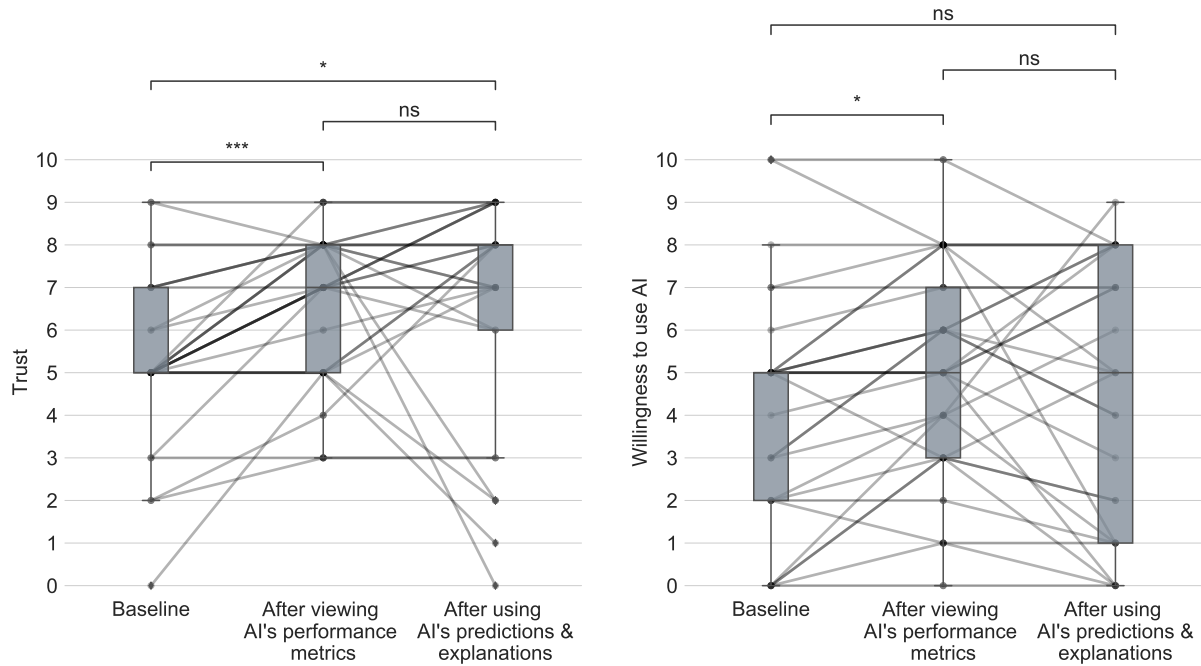
Figure 4: Box plots and changes of participants' trust in the AI (left), and willingness to use AI (right) at the initial baseline, after viewing AI's performance metrics, and after using the AI's predictions and explanations. Both dependent variables are reported on a 0-10 point scale. The lines in between two time points indicate the change for each participant. ns: p > 0.05 , * : 0.01 \leq p \leq 0.05 , ** : 0.001 \leq p \leq 0.01 , *** : 0.0001 \leq p \leq 0.001 .
