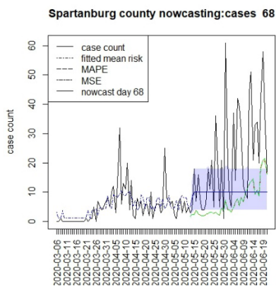
Figure 9 Counterfactual for Spartanburg county T=68
