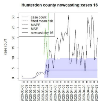
Figure 16 Counterfactual for Hunterdon county T=16
