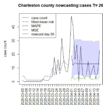
Figure 3 Counterfactual for Charleston county at T=26
