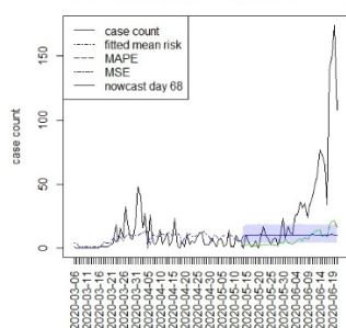
Figure 7 Counterfactual for Charleston county T=68
