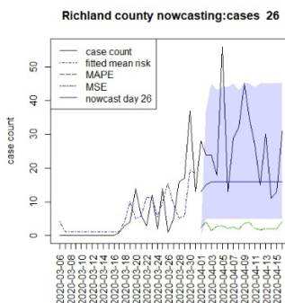
Figure 2 Counterfactual for Richland county at T=26
