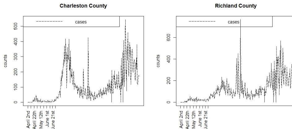
Figure 1 Case count profiles for two South Carolina counties during the first 353 days of the pandemic. The early lockdown dates are shown only.
