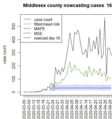
Figure 11 Counterfactual for Middlesex county T=16
