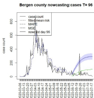
Figure 13 Counterfactual for Bergen county T=96
