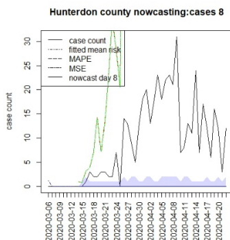
Figure 12 Counterfactual for Hunterdon county T=8
