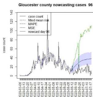
Figure 12 Counterfactual for Gloucester county T=96
