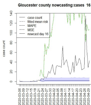
Figure 14 Counterfactual for Gloucester county T=16
