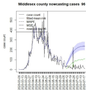
Figure 14 Counterfactual for Middlesex county T=96
