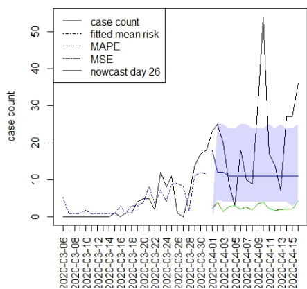
Figure 4 Counterfactual for Greenville county T=26
