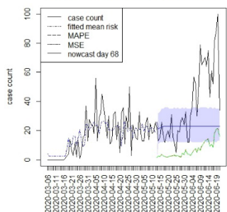
Figure 6 Counterfactual for Richland county T=68
