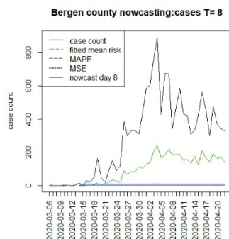
Figure 10 Counterfactual for Bergen county T=8
