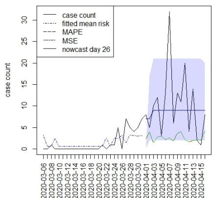
Figure 5 Counterfactual for Spartanburg county at T=26
