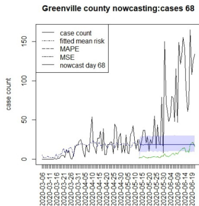
Figure 8 Counterfactual for Greenville county T=68
