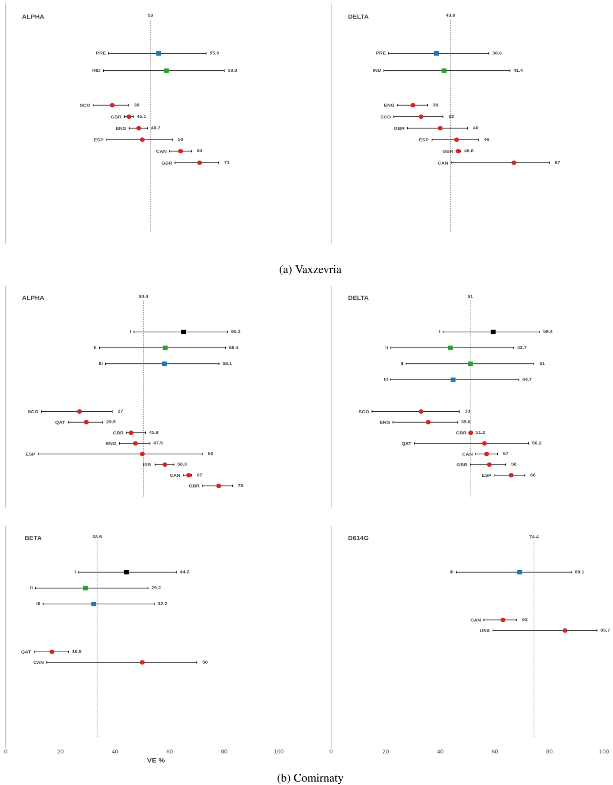
Figure 9: Predictions of one-dose VE against a variant versus VE estimates from indicated countries; see Tables 2 and 3. (a) "Leave-one-variant-out" predictions of Vaxzevria VE, including PRE direct predictions from Vaxzevria data; IND indirect prediction from a Comirnaty-fitted model at Vaxzevria NABTs. (b) Predicted Comirnaty VE. Epoch I: predictions from D614G data. Epoch II: predictions from D614G and another variant; Epoch III: predictions from three other variants, ie, "leave-one-variant-out" predictions.
