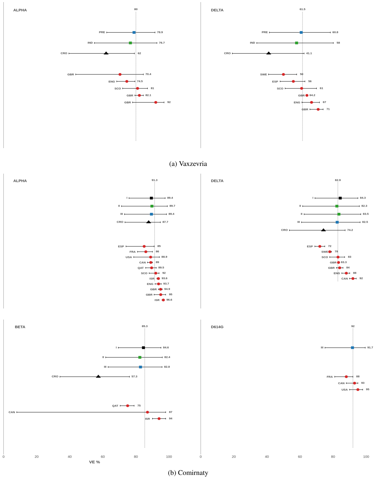
Figure 3: Predictions of two-dose VE against a variant versus VE estimates from indicated countries; see Tables 2 and 3. (a) "Leave-one-variant-out" predictions of Vaxzevria VE, including PRE direct predictions from Vaxzevria data; IND indirect prediction from a Comirnaty-fitted model at Vaxzevria NAbTs; and CRO predictions in [10].(b) Predicted Comirnaty VE. Epoch I: predictions from D614G data. Epoch II: predictions from D614G and another variant; Epoch III: predictions from three other variants, ie, "leave-one-variant-out" predictions; CRO predictions in [10].
