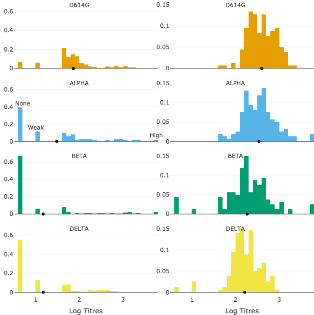
Figure 6: Distributions of \log_{10} -transformed NAbTs after one (Left) and two (Right) Comirnaty doses. Each distribution's geometric mean titre (GMT) is (•). Assay LODs are illustrated for Alpha after one dose: "None", recorded as 5, means no observed neutralisation; "Weak", recorded as 10, means an estimated NAbT below 40; "High", recorded as 5120, means an estimated NAbT above 2560. Data source[15].
