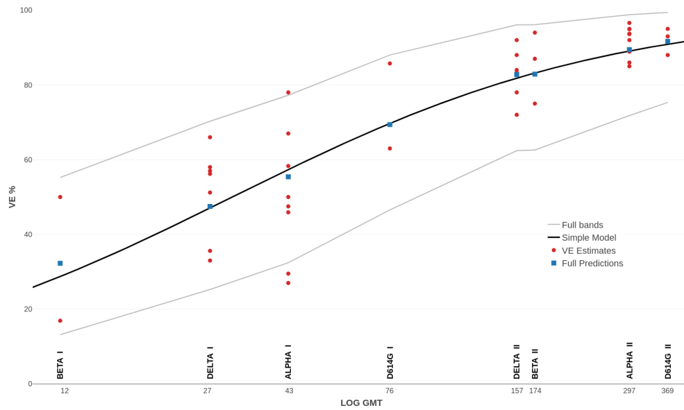
Figure 8: Simplified versus standard models for Comirnaty. The fitted standard model is the same as in Figure 1a. The 95% prediction bands (not shown) for the simplified model are close to those for the standard model.
