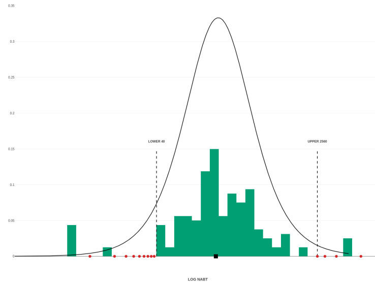
Figure 7: Imputation of NAbTs against Beta for two Comirnaty doses. Logistic pdf was fitted to the censored NAbTs. Nine values (•) were imputed below the LOD, and four (•) above the LOD. GMT is shown(■)
