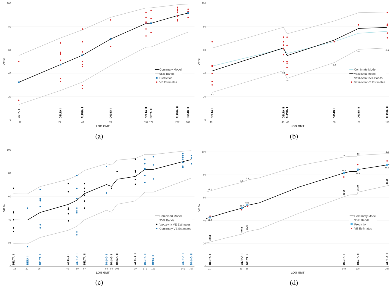
Figure 1: Fitted VE models (2) in adult populations versus \log_{10} GMT, which is labelled on the original scale. As GMT is a scalar summary of NAbTs, each plot is a simplification; see Section A.2. Predictions and VE estimates are per variant and dose (a Roman numeral). (a) Comirnaty VE: direct model. (b) Vaxzevria VE: direct model and indirect model from Comirnaty data, and their prediction differences. (c) Combined VE model fitted to data on both vaccines. (d) Comirnaty model (a) predicts Comirnaty VE against Alpha or Delta in the age subgroups indicated; the GMT is shown for the age subgroups of Legacy; VE estimates are from ref[23]; prediction deviations from them are shown above the prediction band.
