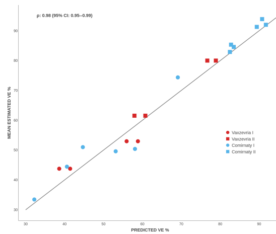
Figure 4: Leave-one-variant-out predictions from the direct and indirect Vaxzevria models and from direct Comirnaty model (including UK-only) versus mean VE estimates per vaccine, dose and variant. The estimated concordance coefficient \rho is displayed on top.
