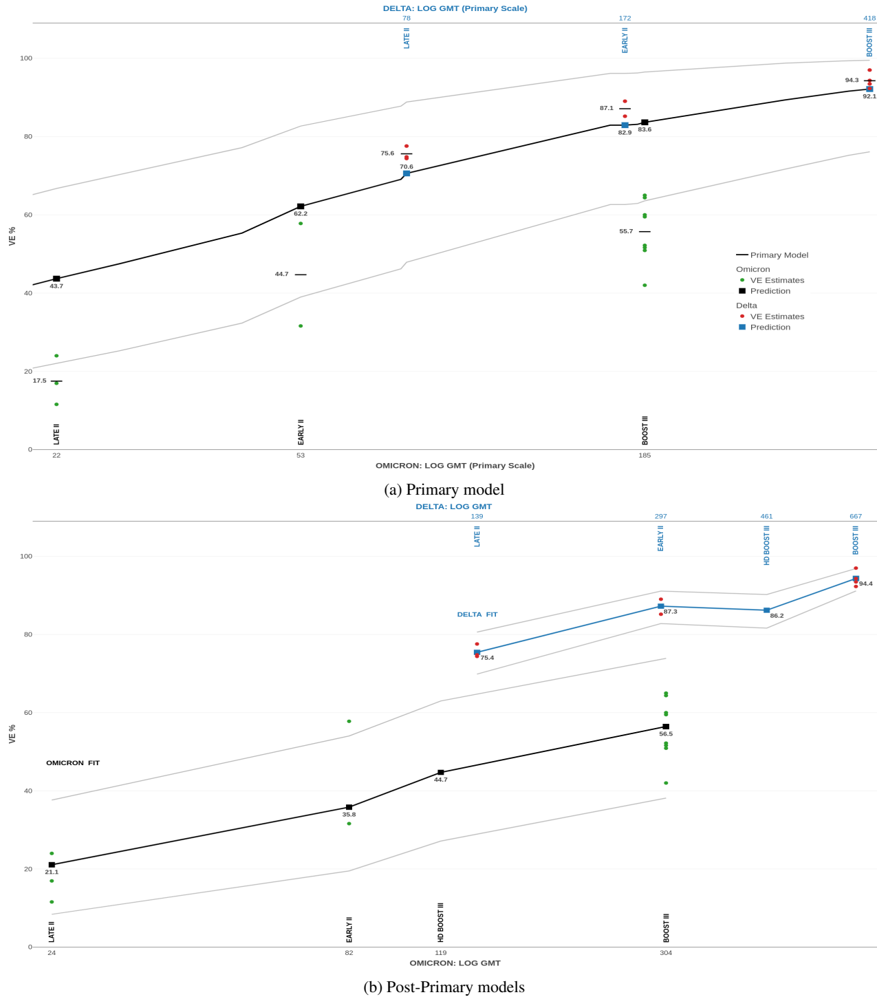
Figure 5: Comirnaty VE for Early group 2–6 weeks after dose II; Late group 12–16 weeks after dose II; Booster group 2–6 weeks after dose III. The top and bottom GMT axes in a plot have the same scale. (a) The Comirnaty model is fitted to "Primary" Legacy NAbTs in seronaive participants. The predictions are based on "Post-Primary" NAbTs[17] divided by 1.51 for Delta and 1.6 for Omicron. (b) Separate models for Comirnaty VE against Delta and Omicron fitted to NAbTs from Post-Primary Legacy. Also shown is predicted VE in haemodialysis (HD) patients 4 weeks after a Comirnaty booster.
