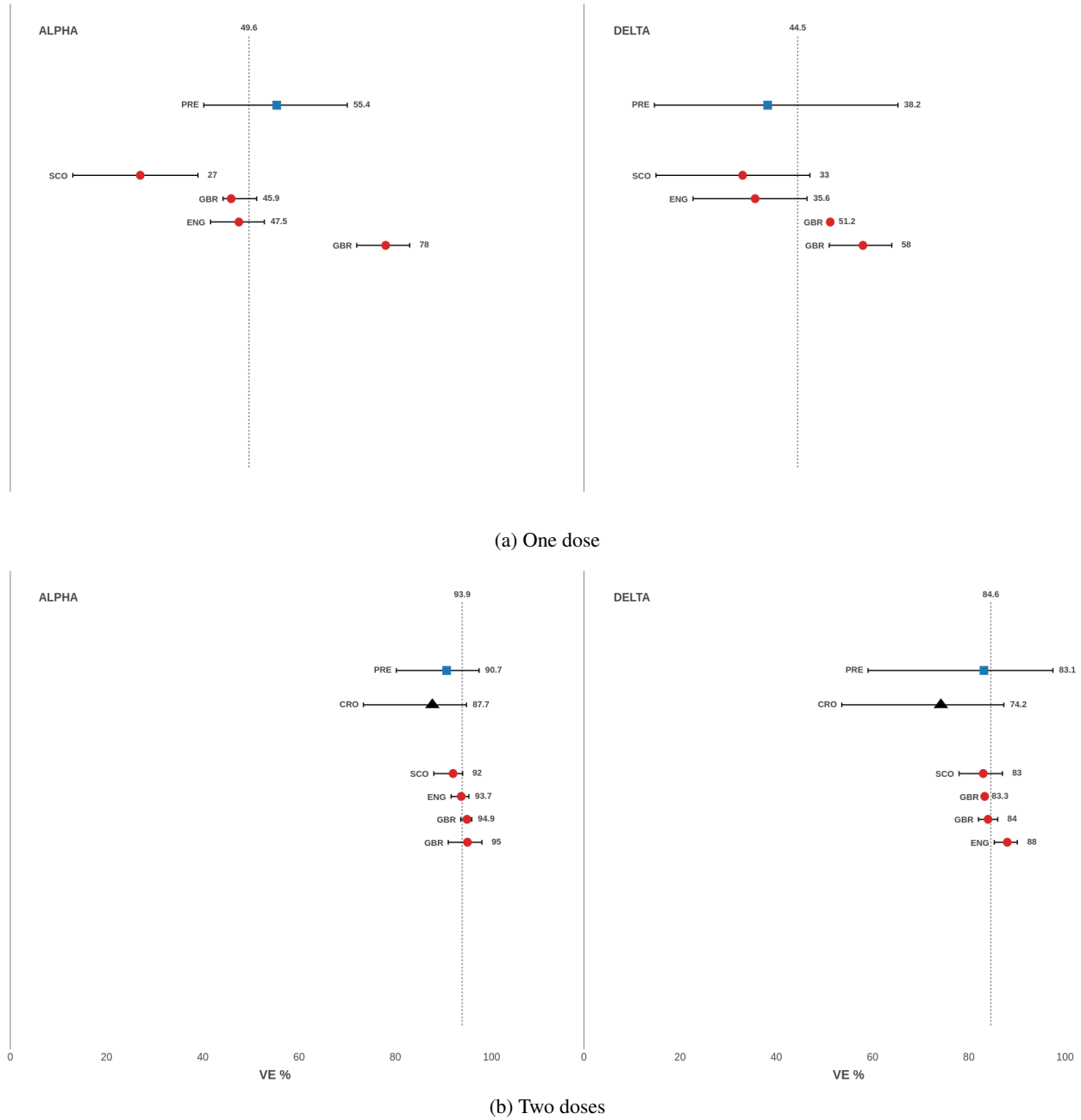
Figure 10: "Leave-one-variant-out" predictions of Comirnaty VE against Alpha or Delta in the UK, from UK data only. PRE obtained predictions; CRO predictions[10], which are not country-specific.
