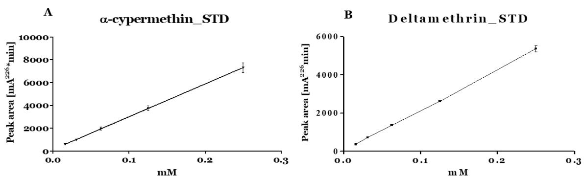
Figure 2: Linear regression of standard curves of \alpha -cypermethrin and deltamethrin.
