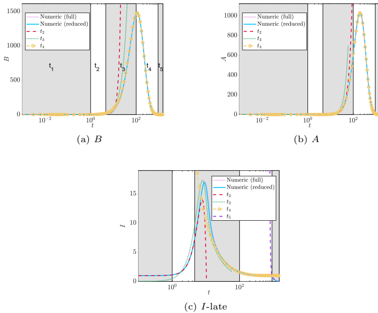
Fig. 2: Comparison of the full model (4), the reduced model (6), and the asymptotic approximations to B , A , and I described in Section 3 with parameters \epsilon = \delta = \kappa_F = \kappa_I = 0.01 , \alpha_L = \alpha_T = \alpha_C = \alpha_I = \lambda_i = 1 , \alpha_V = 2 , and \alpha_B = 3 on a logarithmic non-dimensional time series. For all simulations the initial conditions are L(0) = A(0) = F(0) = I(0) = 1 and V(0) = T(0) = B(0) = C(0) = 0 . We alternate the plot with gray and white patches to indicate the regions where each timescale is valid. Since we have taken \epsilon = 0.01 then the start of each time interval is t_1 = 0.01 , t_2 = 1 , t_3 = 4.64 , t_4 = 100 , and t_5 = 921.03 .
