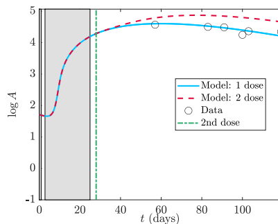
Fig. 5: Comparison of data from Wang et al (2021) to the full model (4) with 1 or 2 doses using the parameters of data set 18 in Tables 2, 3 and second dosage time in Table 4. The alternating patches are the timescale windows in Table 4
