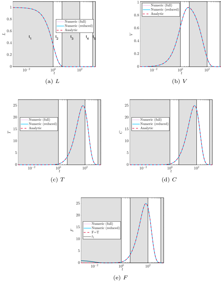
Fig. 1: Comparison of the full model (4), the reduced model (6), and the analytic approximations to L , V , T , C , and F given by (7) and (10) respectively with parameters \epsilon = \delta = \kappa_F = \kappa_I = 0.01 , \alpha_L = \alpha_T = \alpha_C = \alpha_I = \lambda_i = 1 , \alpha_V = 2 , and \alpha_B = 3 on a logarithmic non-dimensional time series. For all simulations the initial conditions are L(0) = A(0) = F(0) = I(0) = 1 and V(0) = T(0) = B(0) = C(0) = 0 . We alternate the plot with gray and white patches to indicate the regions where each timescale is valid. Since we have taken \epsilon = 0.01 then the start of each time interval is t_1 = 0.01 , t_2 = t = 1 , t_3 = 4.64 , t_4 = 100 , and t_5 = 921.03 which are non-dimensional times. For F we note the red-dashed curve represents that quasi-steady limit F = T derived for all timescales beyond t_1 as detailed in section 3.
