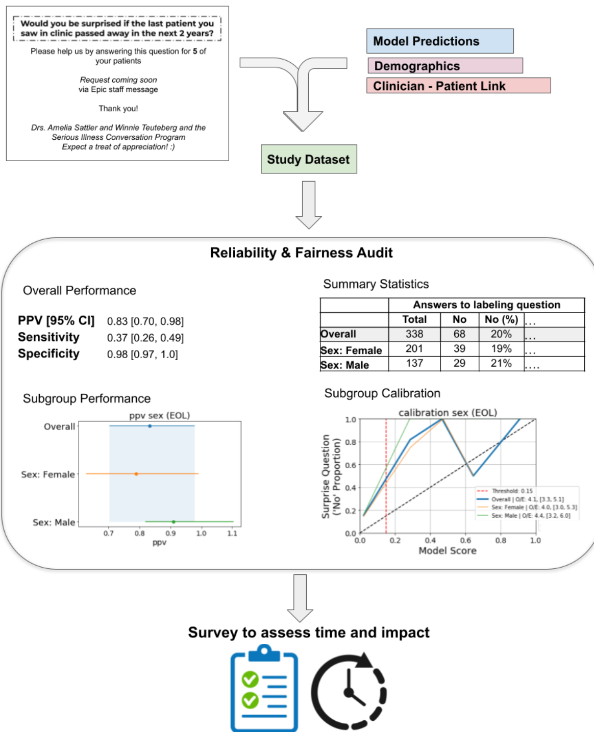
Figure 1: Overview of Audit Process. Results and plots listed are for the Epic End-of-life Index Low Threshold for Primary Care. The “labeling question” under Summary Statistics is “Would you be surprised if this patient passed away in 2 years?”
