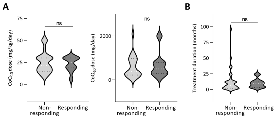
Figure 3 The violin plots of CoQ 10 treatment dose and duration. Two graphs are shown for dosage comparison because CoQ 10 treatment dosages were reported in 2 different units. ns: not significant (Student's t -test).
