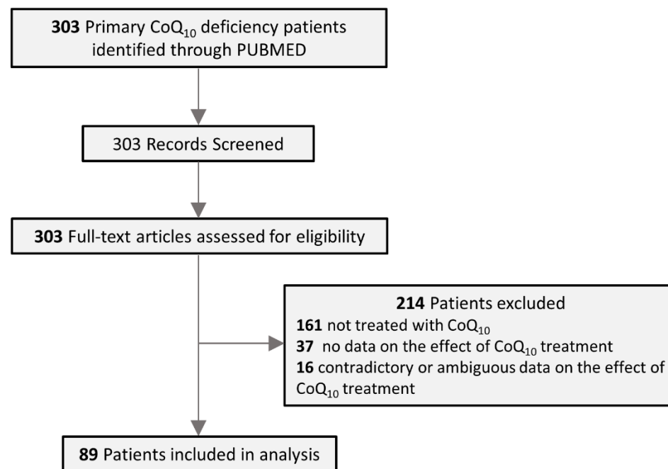
Figure 2 Flow diagram for identification and selection of primary CoQ 10 deficiency patients.
