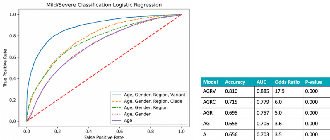
Figure 4. ROC curves after retraining on the expanded October 26 th , 2021 GISAID dataset (left) and updated model performance metrics (right). Previous (Voss et al., 2021) and retrained model performance is superior when genomic mutations are included as features. A general decrease in model performance was observed for the retrained models on the October 2021 dataset in comparison to the previous models, which used the October 20 th , 2020 dataset.
