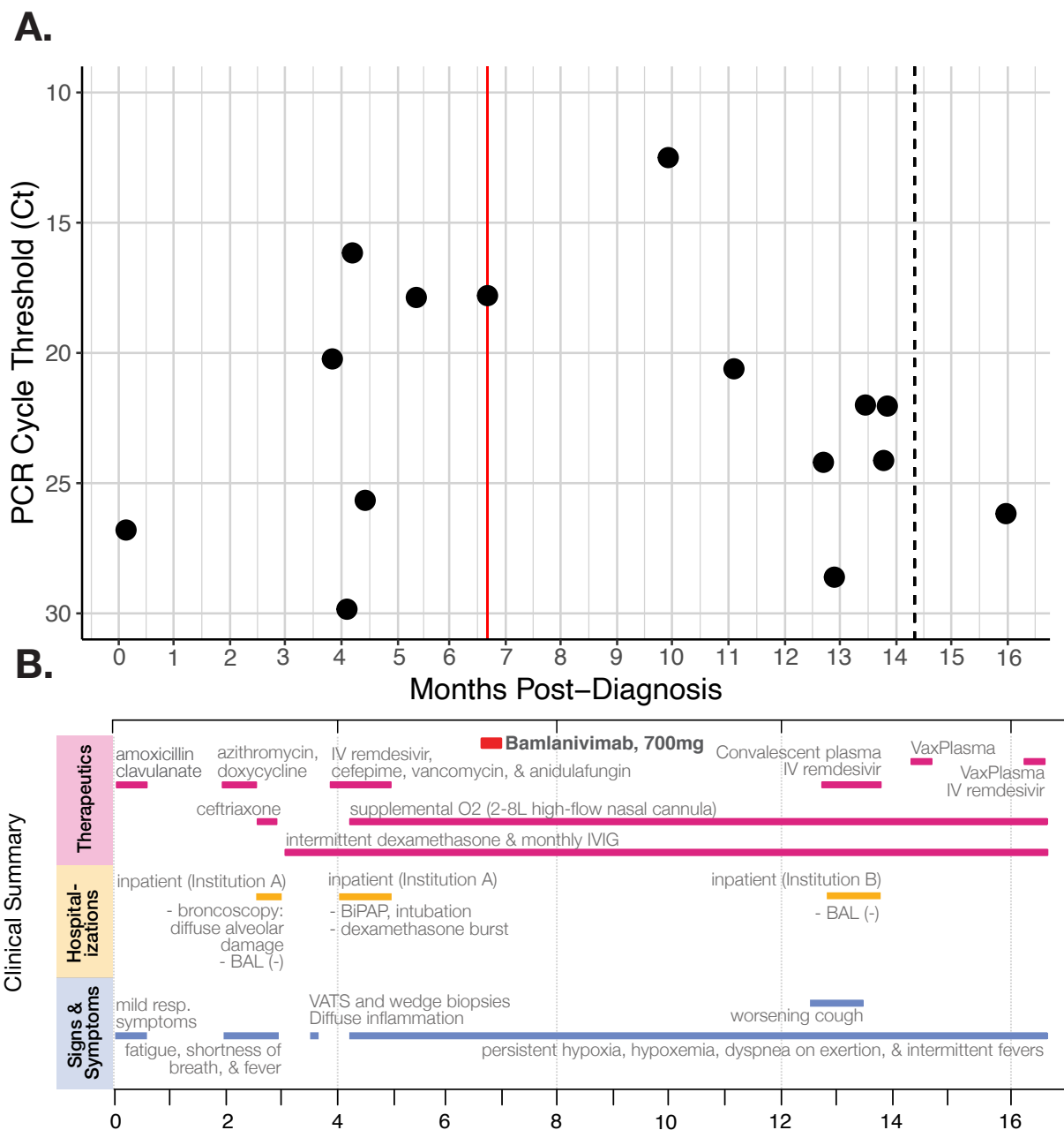
Figure 01. A) RT-qPCR cycle threshold values for patient nasopharyngeal swab specimens collected over almost 16 months of follow-up. The red line marks when the patient received the Bamlanivimab intravenous monoclonal antibody treatment (700mg). The dotted line in month 14 indicates a positive PCR test but no available Ct value. Note that Ct values are inverted to correspond with the inverse relationship between PCR Ct threshold value and nasal RNA copy number. B) Timeline of clinically relevant information for the patient's chronic infection, including symptoms, therapeutics, and hospitalizations.
