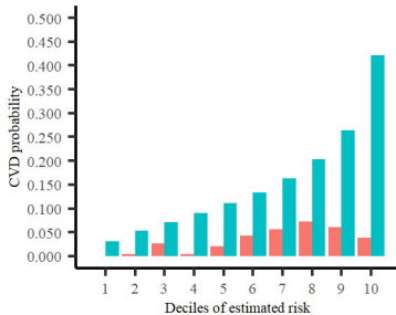
Framingham CVD model
