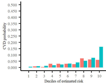
Wu's simplified model
