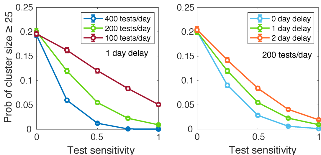
367 Fig 3: Results of a Monte Carlo simulation of infection transmission on a network of 1600 368 individuals. We track the probability that a single starting infection seeds a cluster of 25 or 369 more infections. We compare a baseline protocol that has a capacity of 200 tests per day and 370 a delay in reporting of one day (green), with variations having higher or lower capacities or 371 delays (see legend). Error bars represent SEM values over 5000 replicate simulations.
