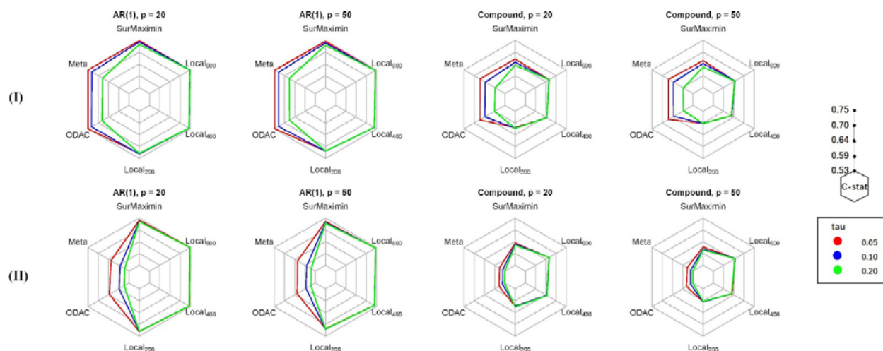
Figure 2: Average C-statistics under settings (I) and (II) with \Sigma being either AR(1) or compound symmetry; p = 20 or 50; and \tau = 0.05, 0.10 , or 0.20 (local coefficients heterogeneity) for predicting survival in the target population with risk models trained by SurvMaximin, (Meta), ODAC, as well as supervised penalized Cox regression with n_Q = 200, 400, 600 labeled target data (Local 200 , Local 400 , Local 600 ).
