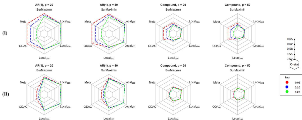
Figure S1: Average C-statistics under settings (I) and (II) with \Sigma being either AR (I) or compound symmetry, p = 20 or 50 , and \tau = 0.05, 0.1, 0.2 (local coefficients heterogeneity) for predicting survival in the target population with risk models trained by SurMaximin, Meta, and ODAC, as well as supervised penalized Cox regression with n_Q = 200, 400, 600 labeled target data ( Local_{200}, Local_{400}, Local_{600} ).
