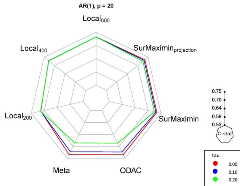
Figure S2: Average C-statistics under settings (I) with \Sigma being AR (1), p = 20 , and \tau = 0.05, 0.1, 0.2 (local coefficients heterogeneity) for predicting survival in the target population with one missing feature based on risk models trained by SurvMaximin, SurvMaximinproject, Meta, and ODAC, as well as supervised penalized Cox regression with n_Q = 200, 400, 600 labeled target data (Local 200 , Local 400 , Local 600 ).
