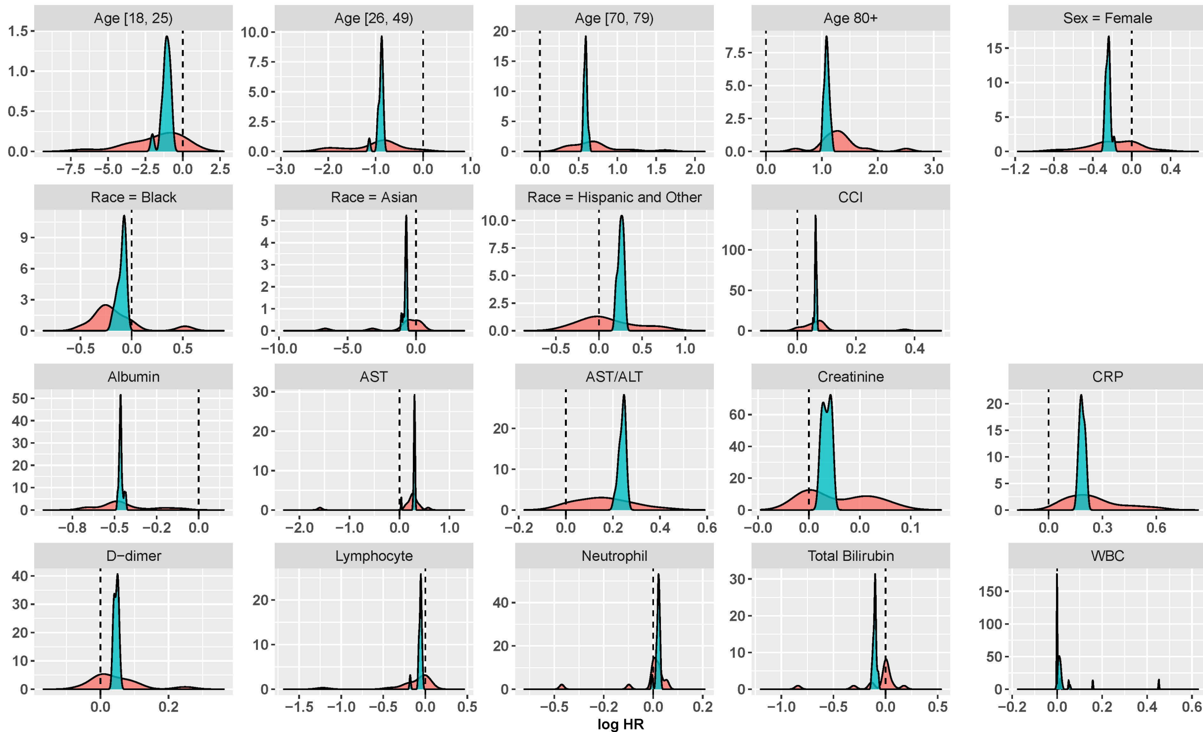
Method ■ Local ■ SurvMaximin
