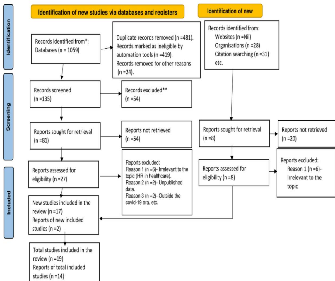
Figure 1: PRISMA 2020 diagram
