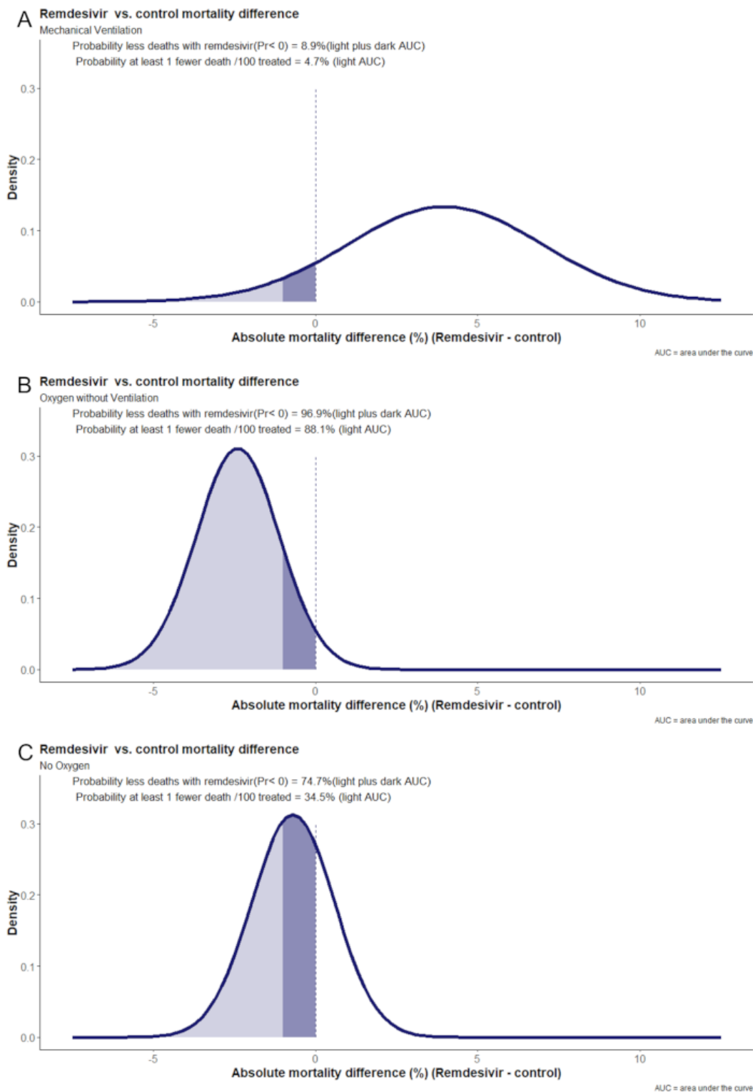
Figure 2 – Probability density functions for combined posterior distributions of the included remdesivir trials. (A) Mechanical ventilation. (B) Supplemental oxygen without mechanical ventilation. (C) No oxygen support.
