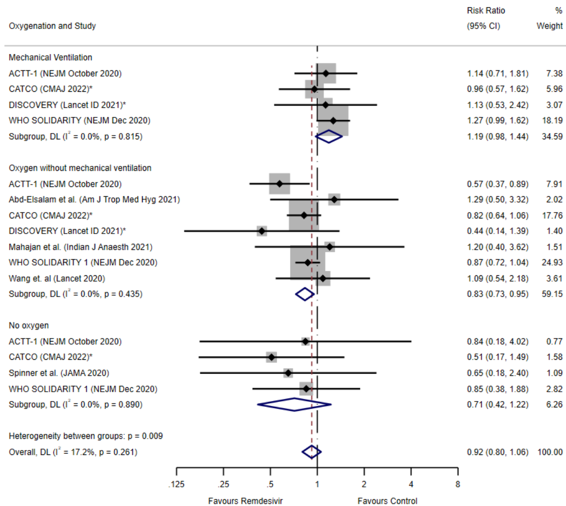
Figure 1 – Random Effects Meta-Analysis
