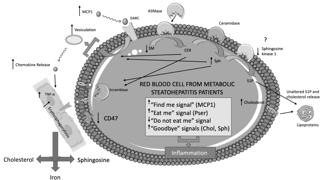
Figure 3. Schematic mechanism of inflammation pathways in NASH. In NASH, there is increased serum acid sphingomyelinase (ASMase) 30 , which breaks sphingomyelin (SM) to phosphocholine and ceramide (CER). This enzyme can act on the erythrocyte membrane 31 leading to reduction of sphingomyelin 34 and release of microvesicles 32 . Microvesicles release chemokines such as MCP1, which could activate macrophages 14 . Erythrocyte sphingolipid metabolism can result in the formation of sphingosine (Sph) 32 and sphingosine 1-phosphate (S1P) 9 . However, it has previously been shown that erythrocyte-conditioned media do not contain elevated S1P, possibly because of inhibition of sphingosine kinase 1. Sphingosine accumulation in red blood cells triggers eryptosis 35 , through activation of calcium channels and subsequent activation of scramblase. Phosphatidylserine exposure 13 along with reduced membrane CD47 levels can promote erythrophagocytosis in the liver. Once erythrophagocytosis has occurred, increased membrane cholesterol and sphingosine, along with iron disposition could augment inflammation. This figure was created using Servier Medical
