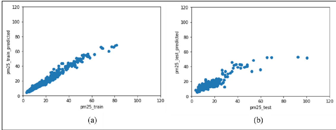
356 Figure 88. Predicted PM_{2.5} versus the measured PM_{2.5} levels ( 10^{-3} \text{ mol/m}^2 ) from the (a) 357 training and (b) testing datasets using RF.
