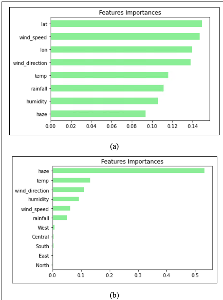
369 Figure 9. Feature importance in (a) NO_2 and (b) PM_{2.5} modelling using RF.
